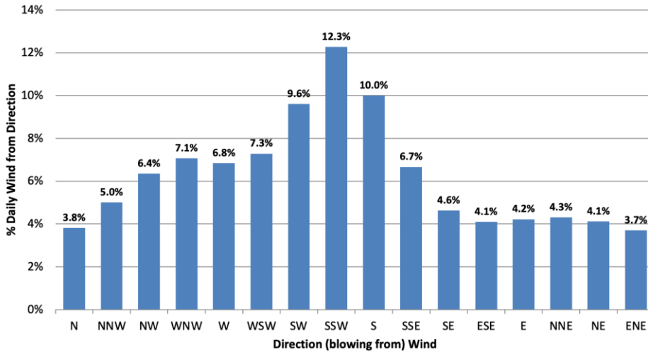
Figure 1. 25-year Average Illinois Wind Direction 57
