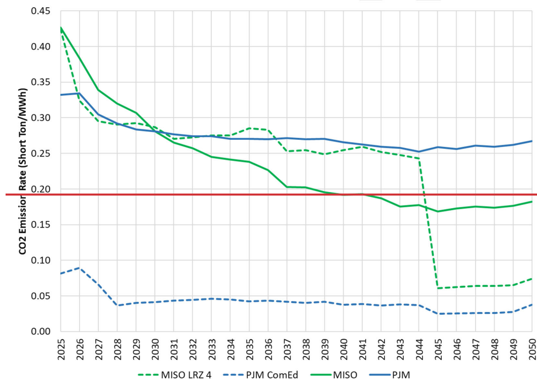
Figure 8-14: CO 2 Emission Rate
