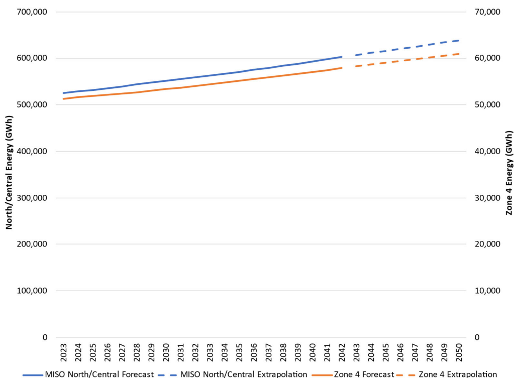
Figure 8-3: Annual Energy Forecast, MISO 674
