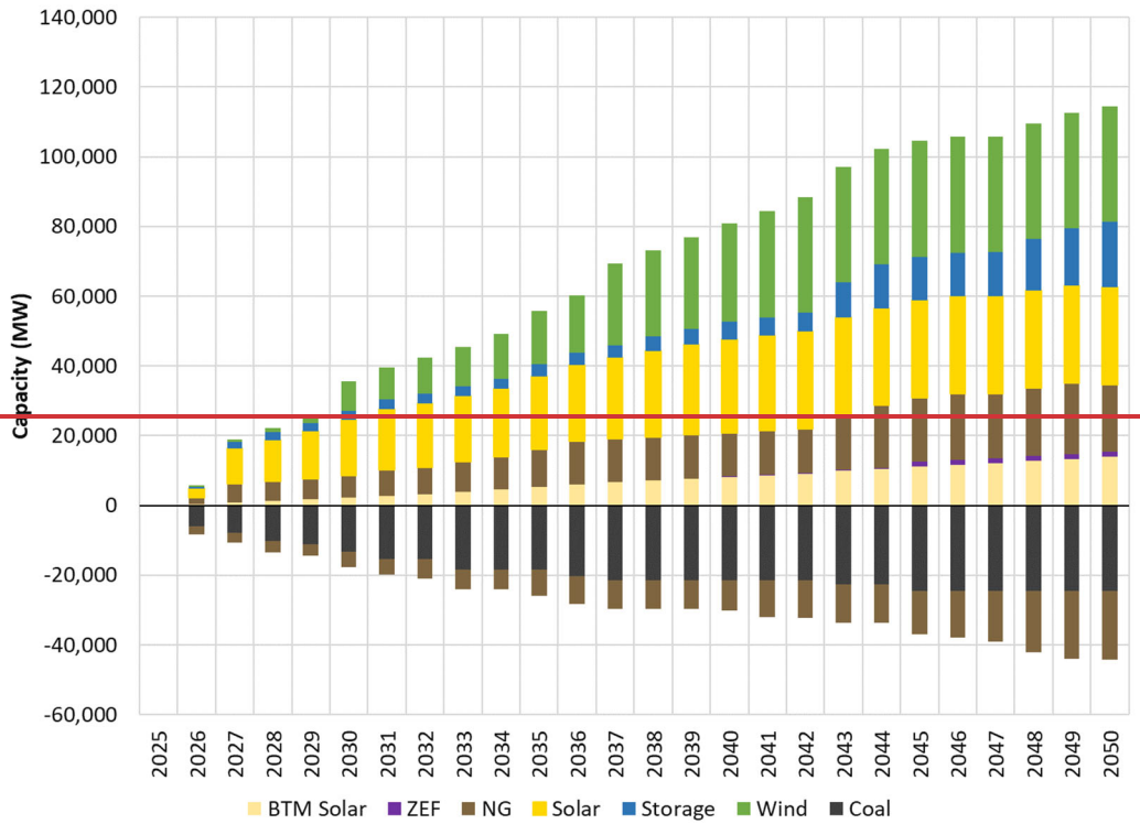
Figure 8-10: Cumulative MISO Resource Addition and Retirement
