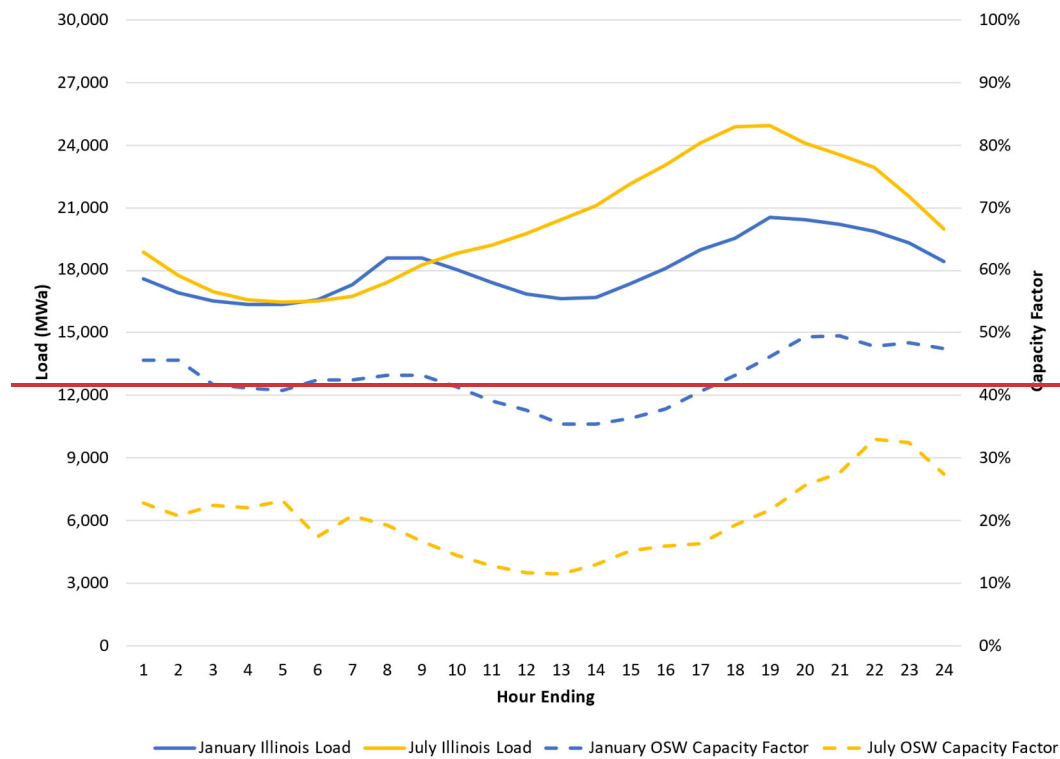
Figure 8-18: Load and Offshore Wind Average Profiles 754
