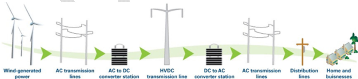
Figure 7-11: HVDC Power Conversion
