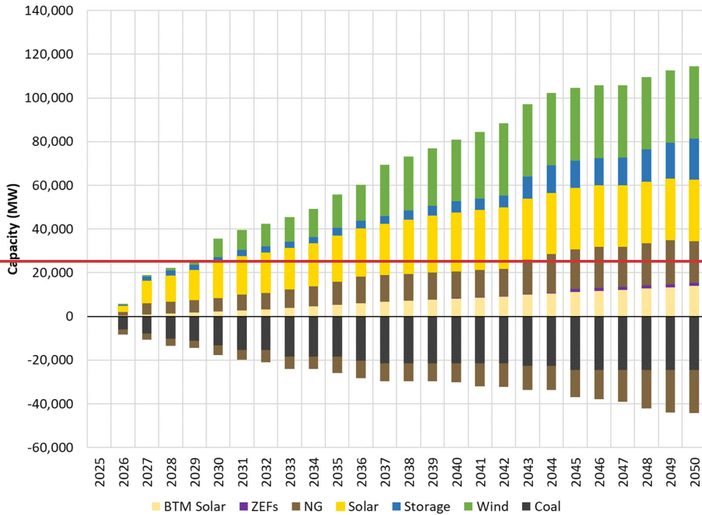
Figure 8-11: Cumulative PJM Resource Addition and Retirement
