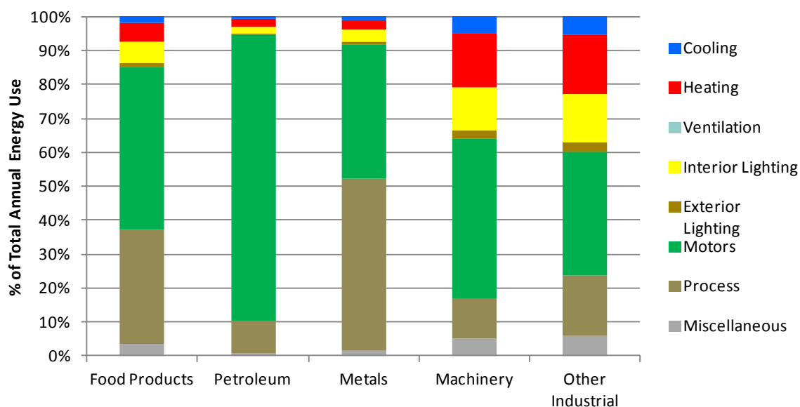
Figure 3-19 Breakdown of Industrial Electricity Use by End Use and Segment (2011)
