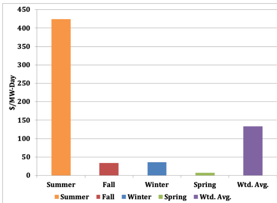
Figure 5-7: 2026-2027 Delivery Year Seasonal PRA Results for MISO Zone 4
