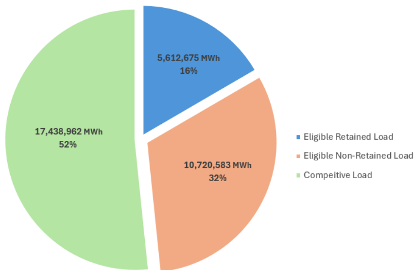
Figure 3-1: Ameren Illinois' Forecast Retail Customer Load Breakdown, Delivery Year 2027-2028 114
