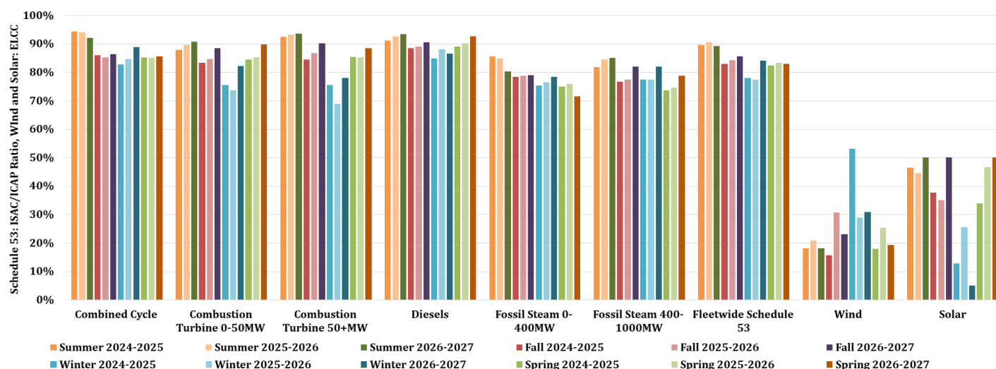
Figure 5-6: Schedule 53 Seasonal Resource ISAC/ICAP; Wind and Solar ELCCs 190
