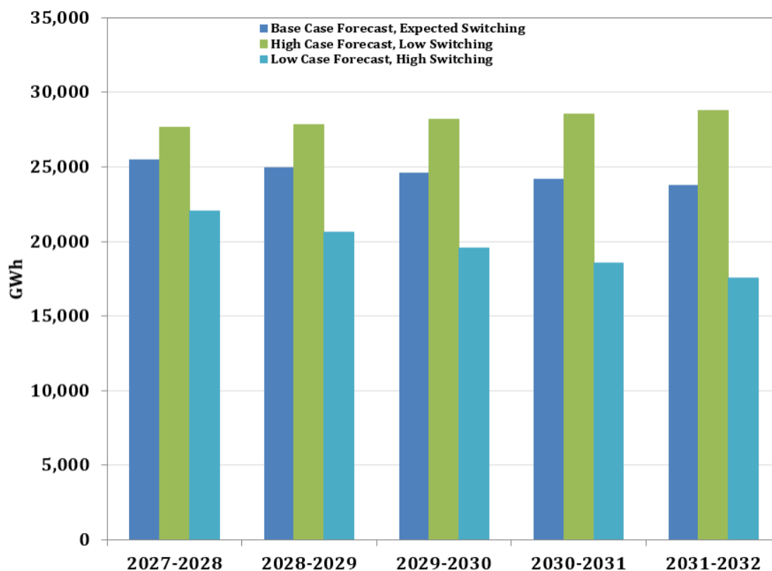
Figure 3-12: Supply Obligation in ComEd's Forecast Scenarios
