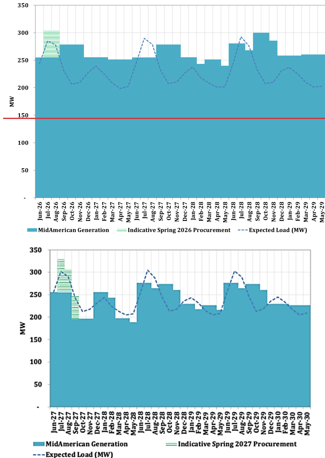
Figure 7-5: MidAmerican Peak Energy Supply Portfolio and Load 270
