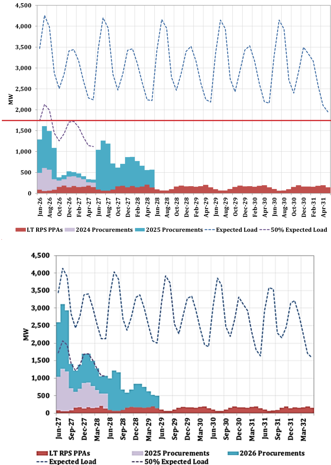
Figure 4-2: ComEd's On-Peak Supply Gap - June 2026-2027-May 2031-2032 period - Base Case Load Forecast
