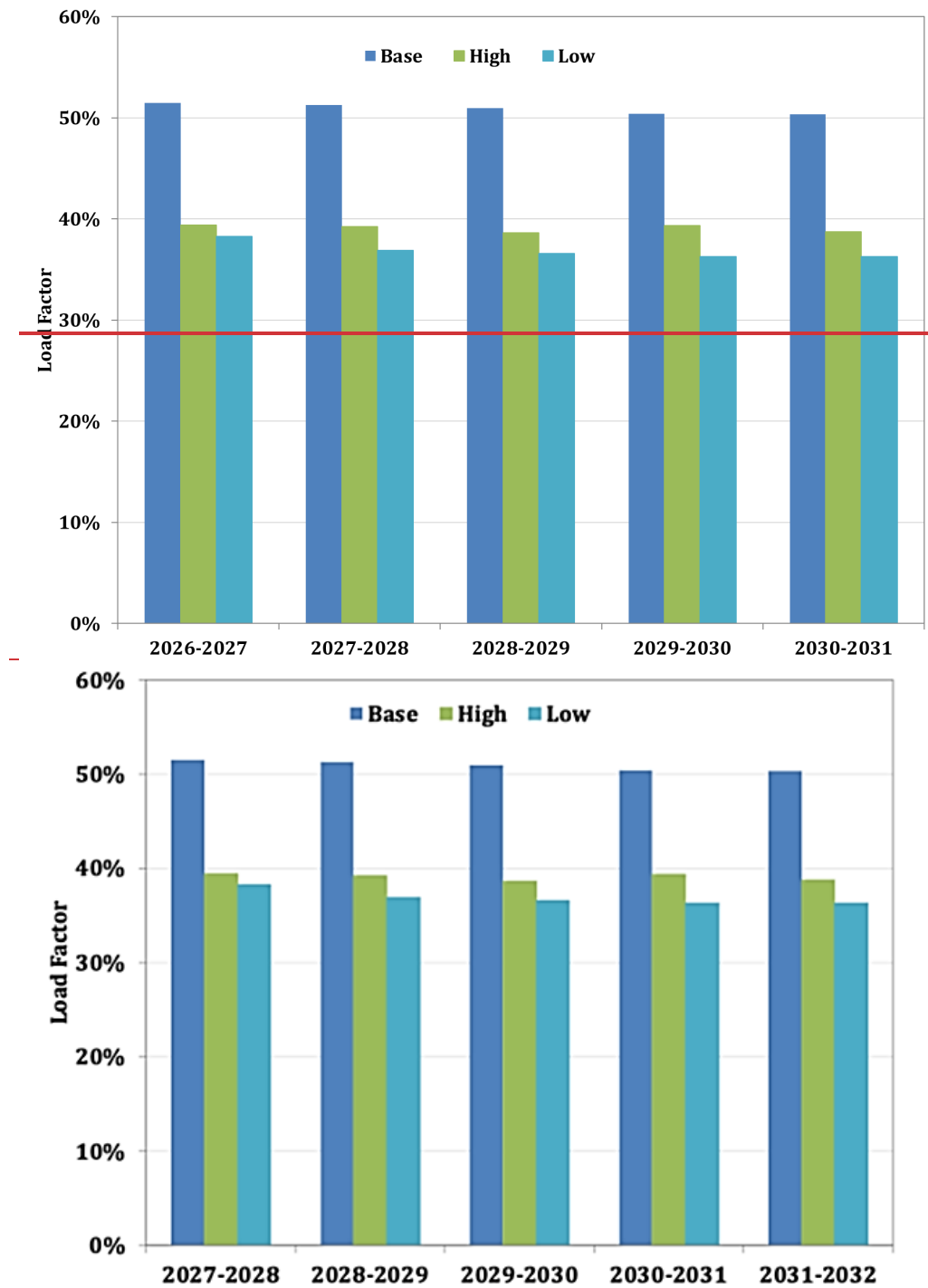
Figure 3-15: Load Factor in ComEd's Forecasts Scenarios
