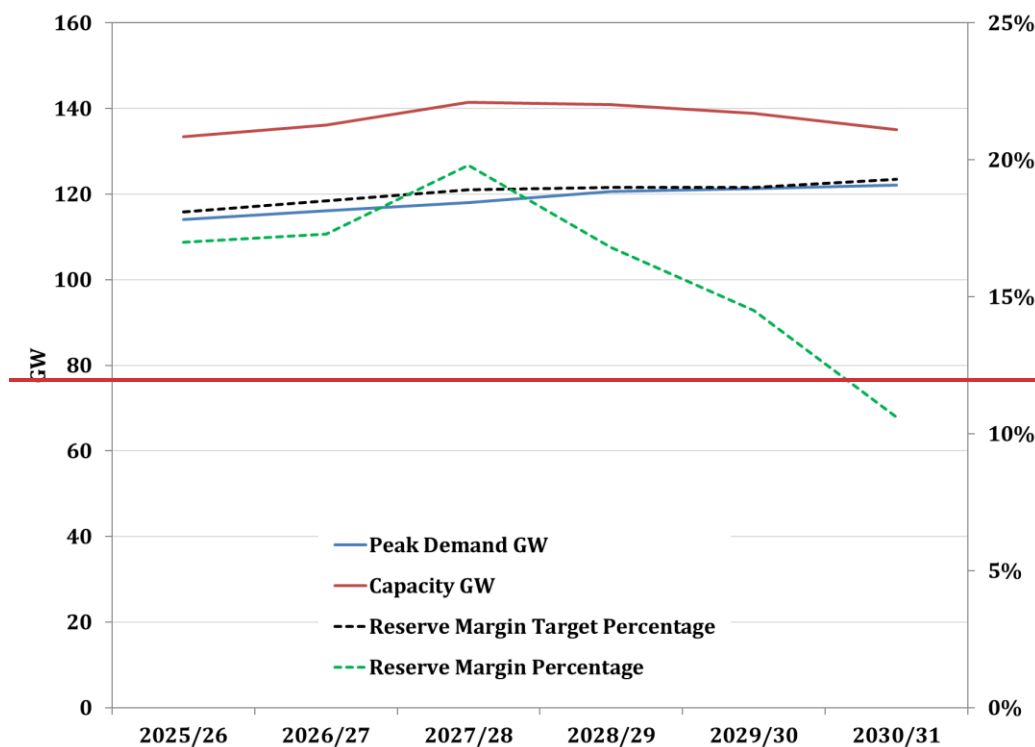
Figure 5-3: NERC Projection of Supply and Demand for the Delivery Years 2025-2026 to 2030-2031 173
