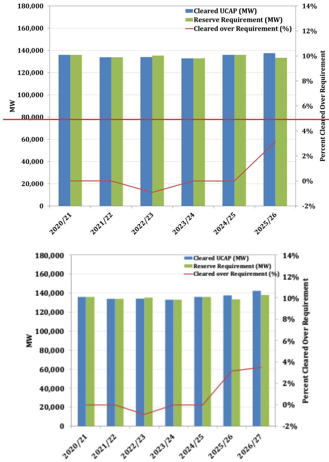
Figure 5-4: MISO Historical PRA Cleared UCAP and Reserve Margin
