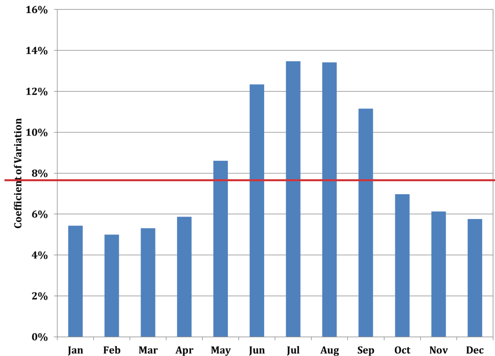
Figure 3-23: Coefficient of Variation of Daily Peak-Period Loads
