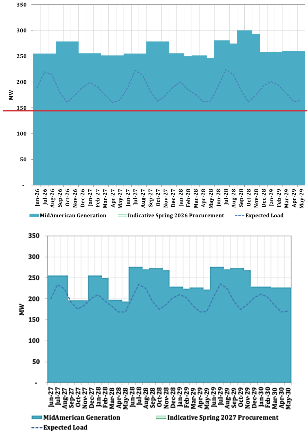
Figure 7-6: MidAmerican Off-Peak Energy Supply Portfolio and Load
