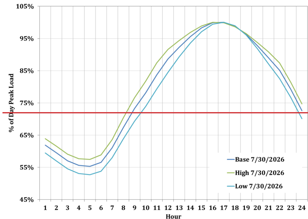
Figure 3-20: Sample Daily Load Shape, Summer Day in MidAmerican's Forecasts
