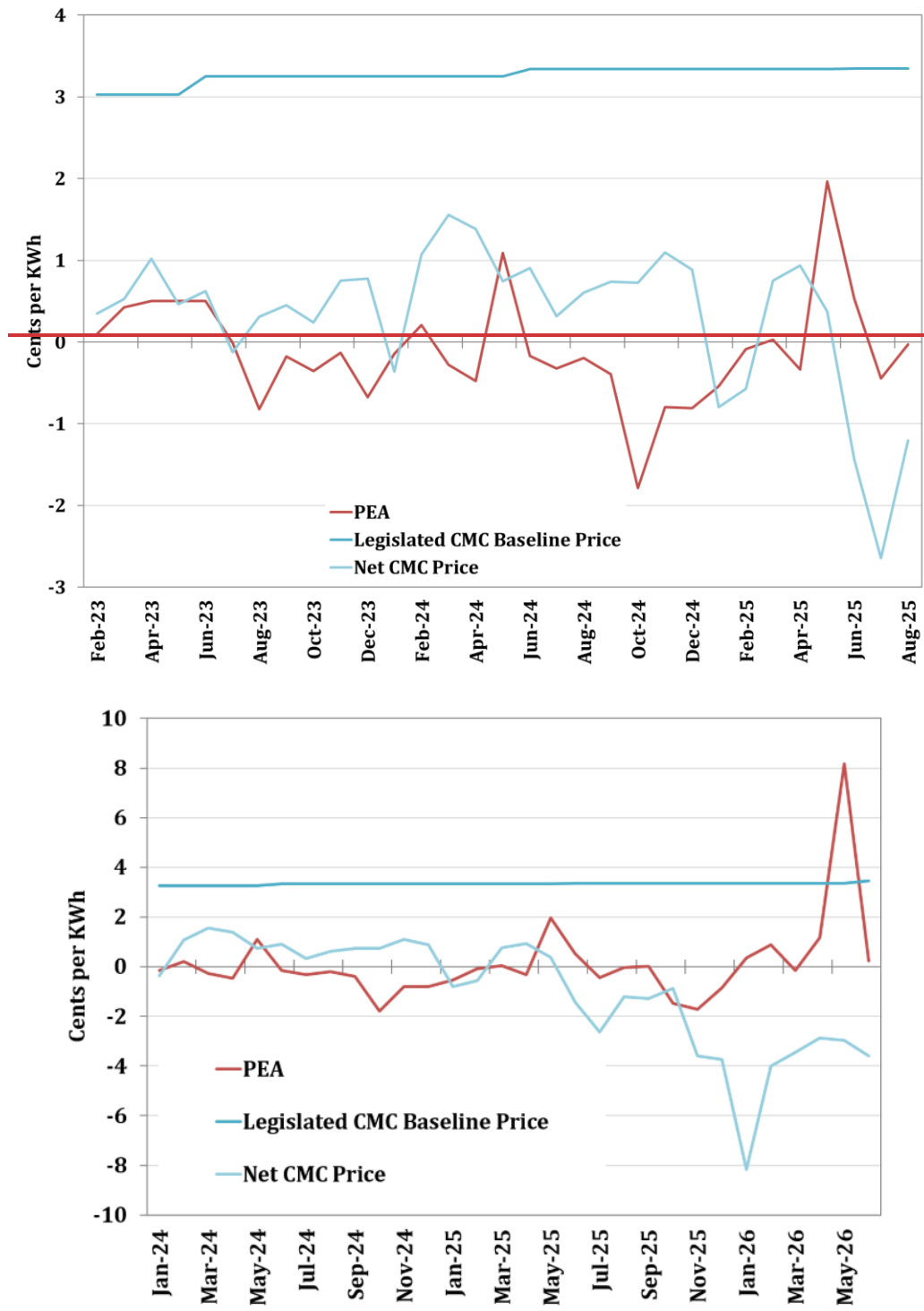
Figure 6-2: Monthly Purchased Electricity Adjustment Factors vs. CMC Baseline and CMC Net Prices
