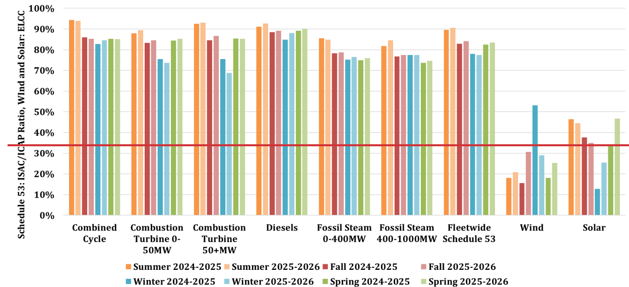
Figure 5-6: Schedule 53 Seasonal Resource ISAC/ICAP; Wind and Solar ELCCs 206
