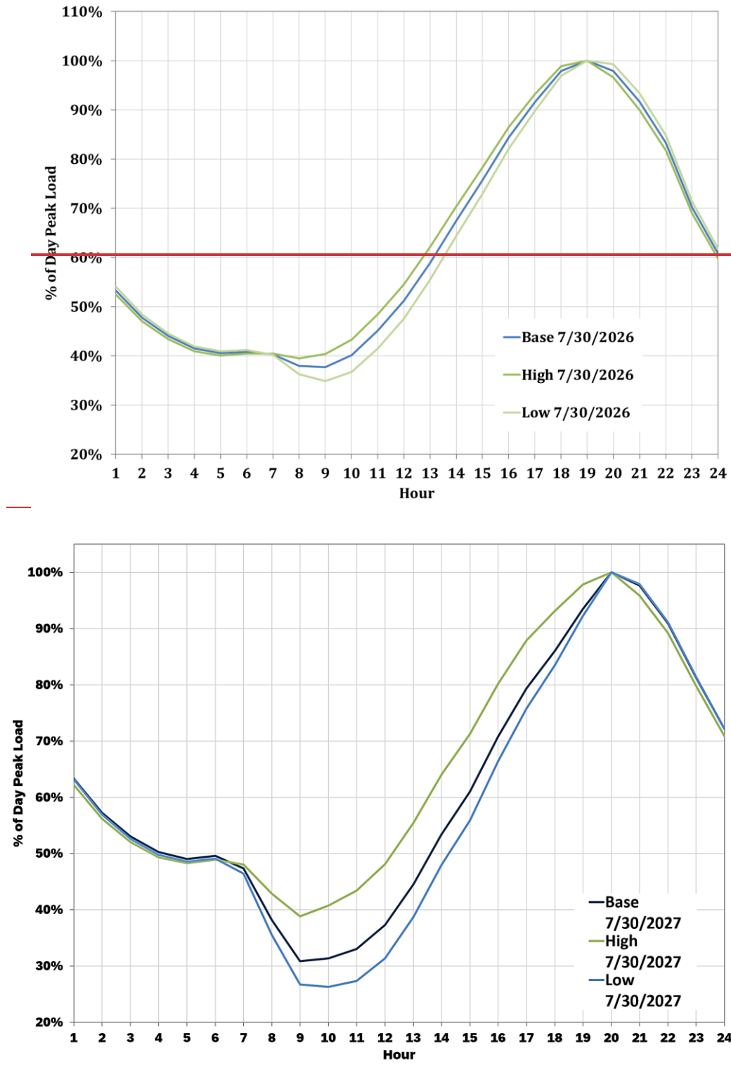
Figure 3-5: Sample Daily Load Shape, Summer Day in Ameren Illinois' Forecasts
