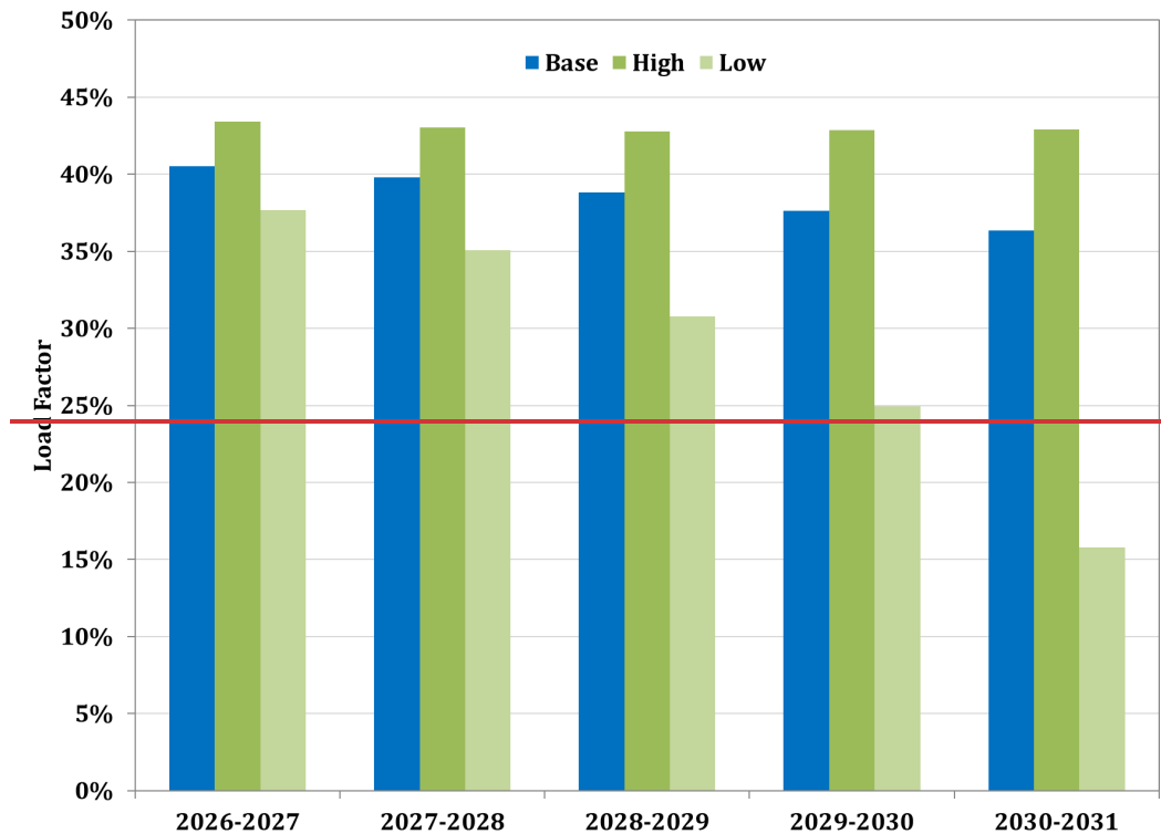
Figure 3-7: Load Factor in Ameren Illinois' Forecast Scenarios
