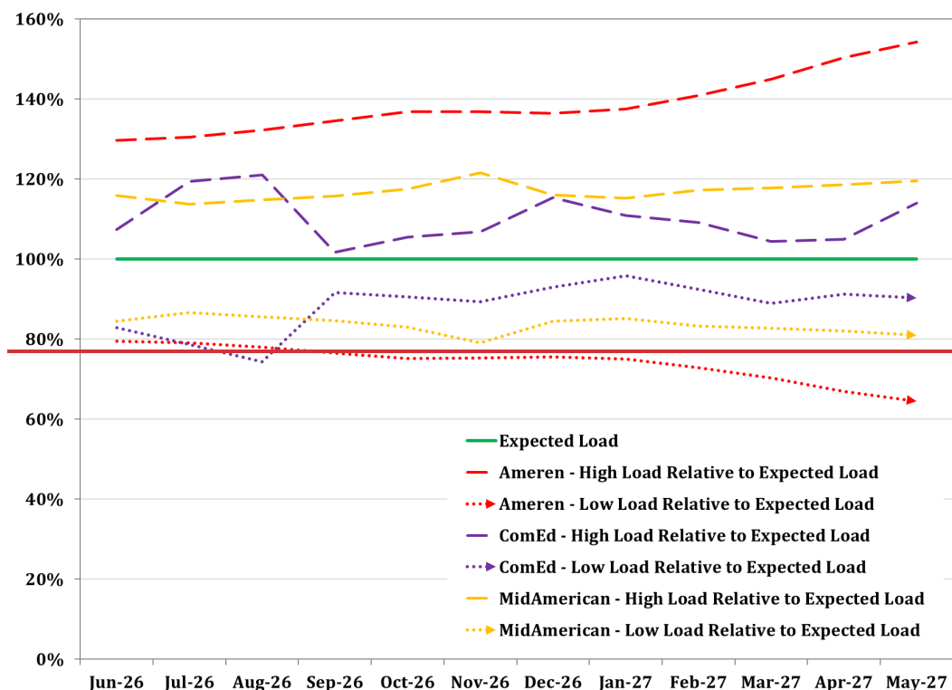
Figure 3-25: Comparison of Ameren Illinois, ComEd, and MidAmerican High and Low Load Forecasts for Delivery Year 2026-2027-2028
