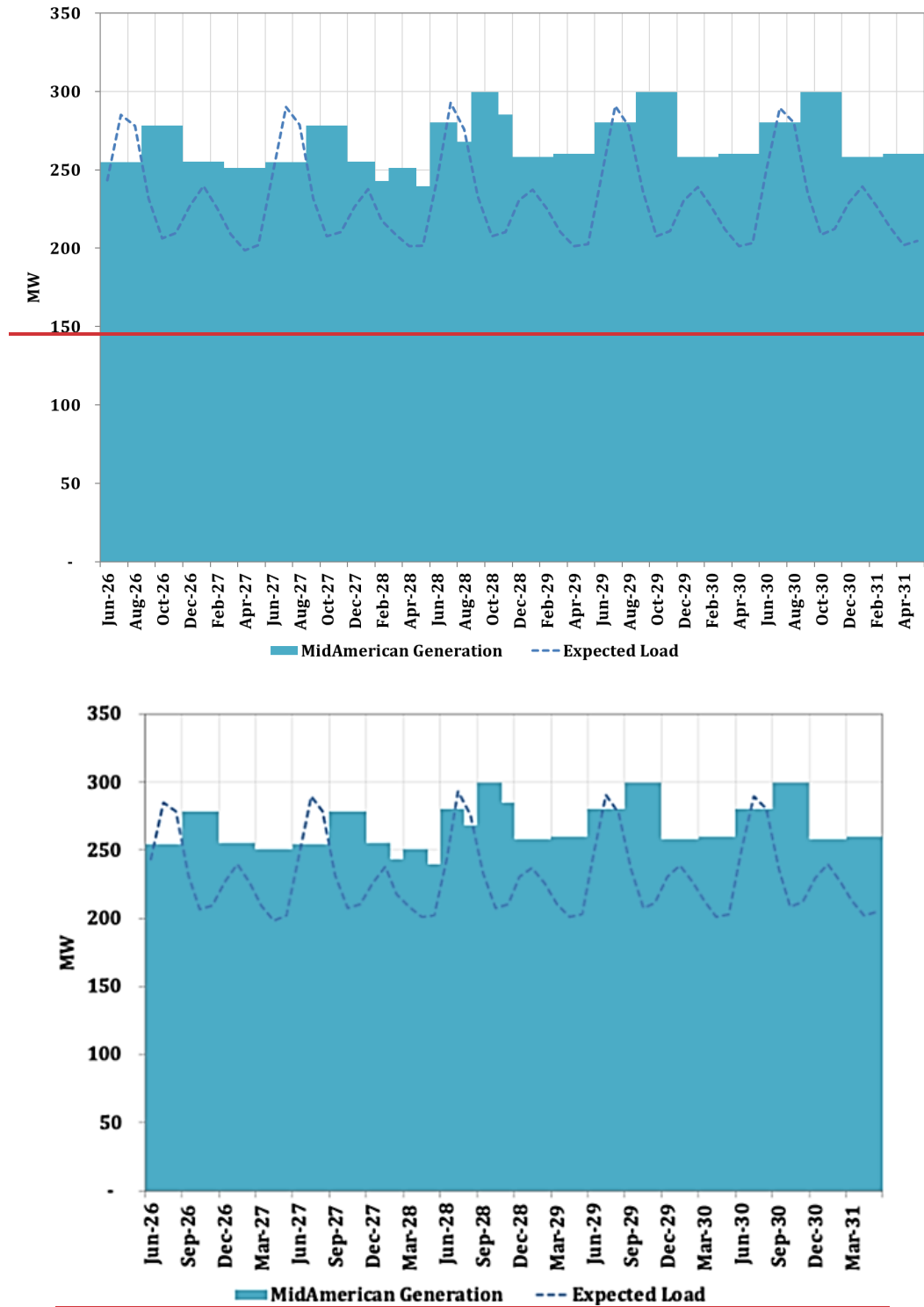
Figure 4-3: MidAmerican's On-Peak Supply Gap - June 2026-2027-May 2031-2032 period - Base Case Load Forecast
