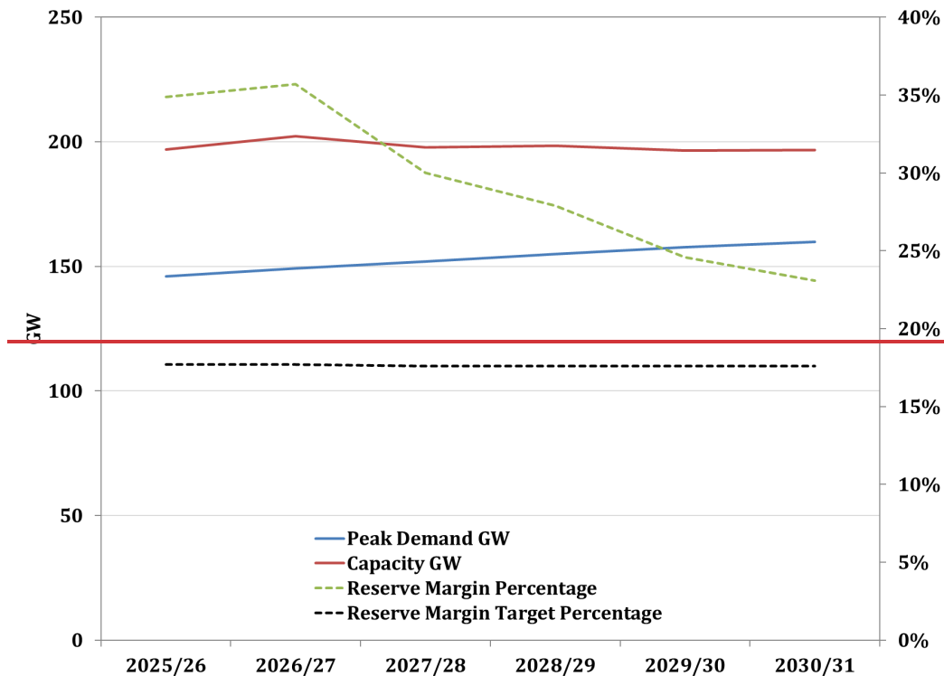
Figure 5-1: NERC Projection of Supply and Demand for Delivery Years 2025-2026 to 2030-2031 164
