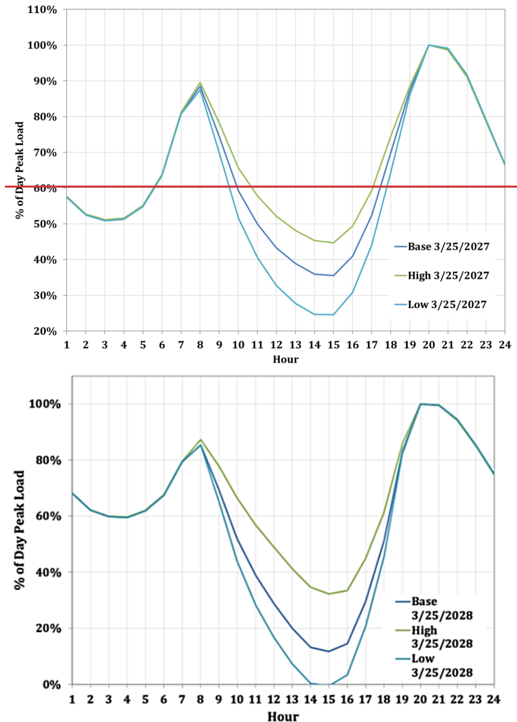
Figure 3-6: Sample Daily Load Shape, Spring Day in Ameren Illinois' Forecasts
