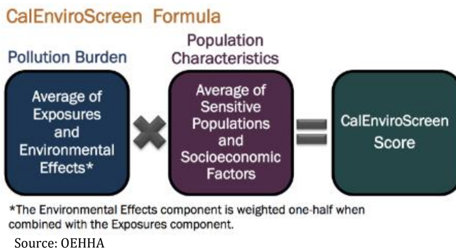
Figure 8-7: CalEnviroScreen Formula
