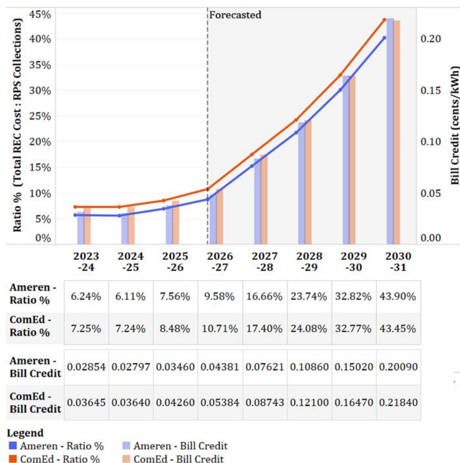
Figure 6-1: Actual & Forecast Self-Direct Program Bill Credit Rates 356
