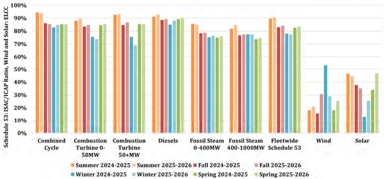
Figure 5-6: Schedule 53 Seasonal Resource ISAC/ICAP; Wind and Solar ELCCs 163
