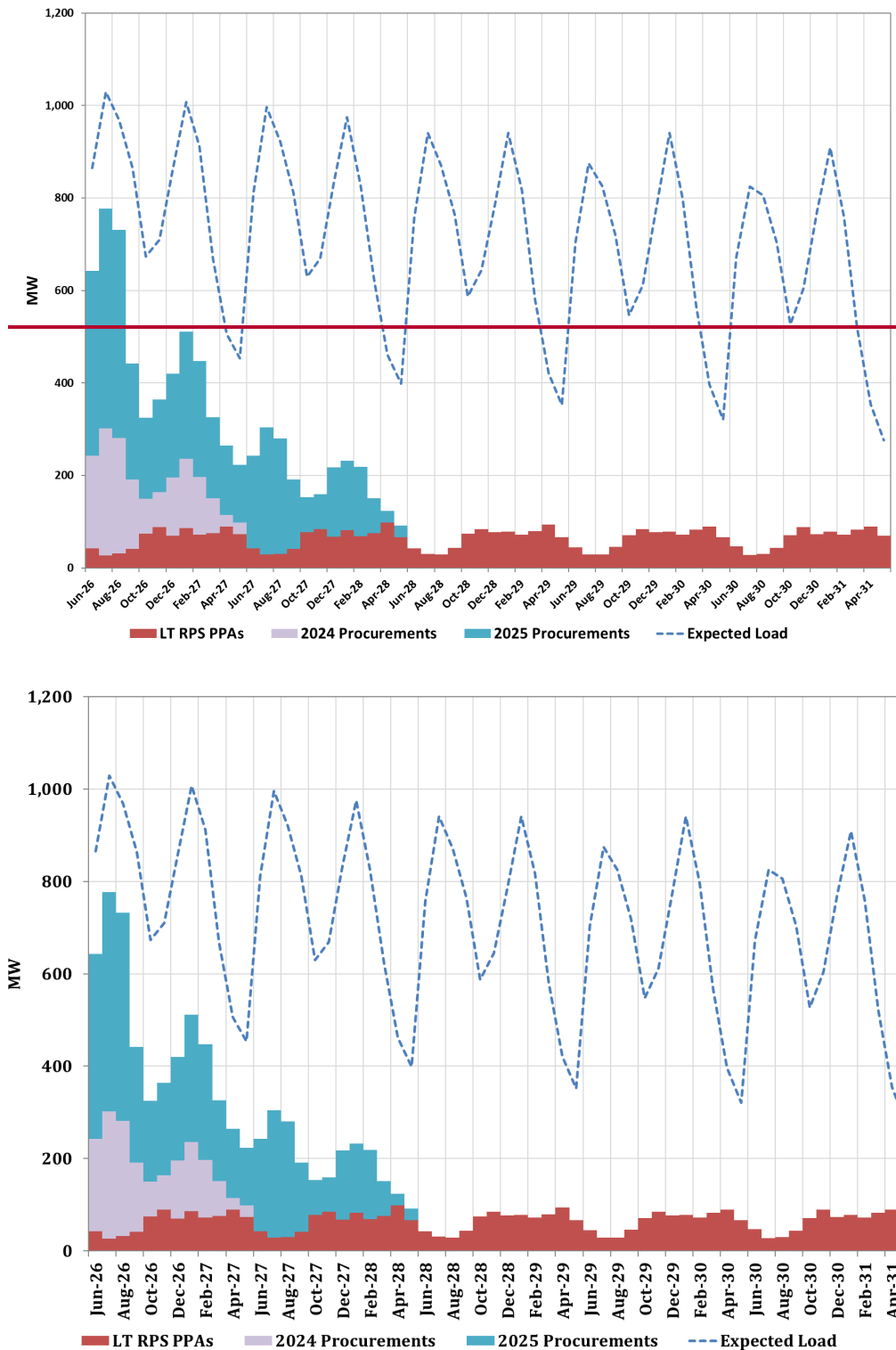
Figure 4-1: Ameren Illinois' On-Peak Supply Gap - June 2026-May 2031 Period - Base Case Load Forecast
