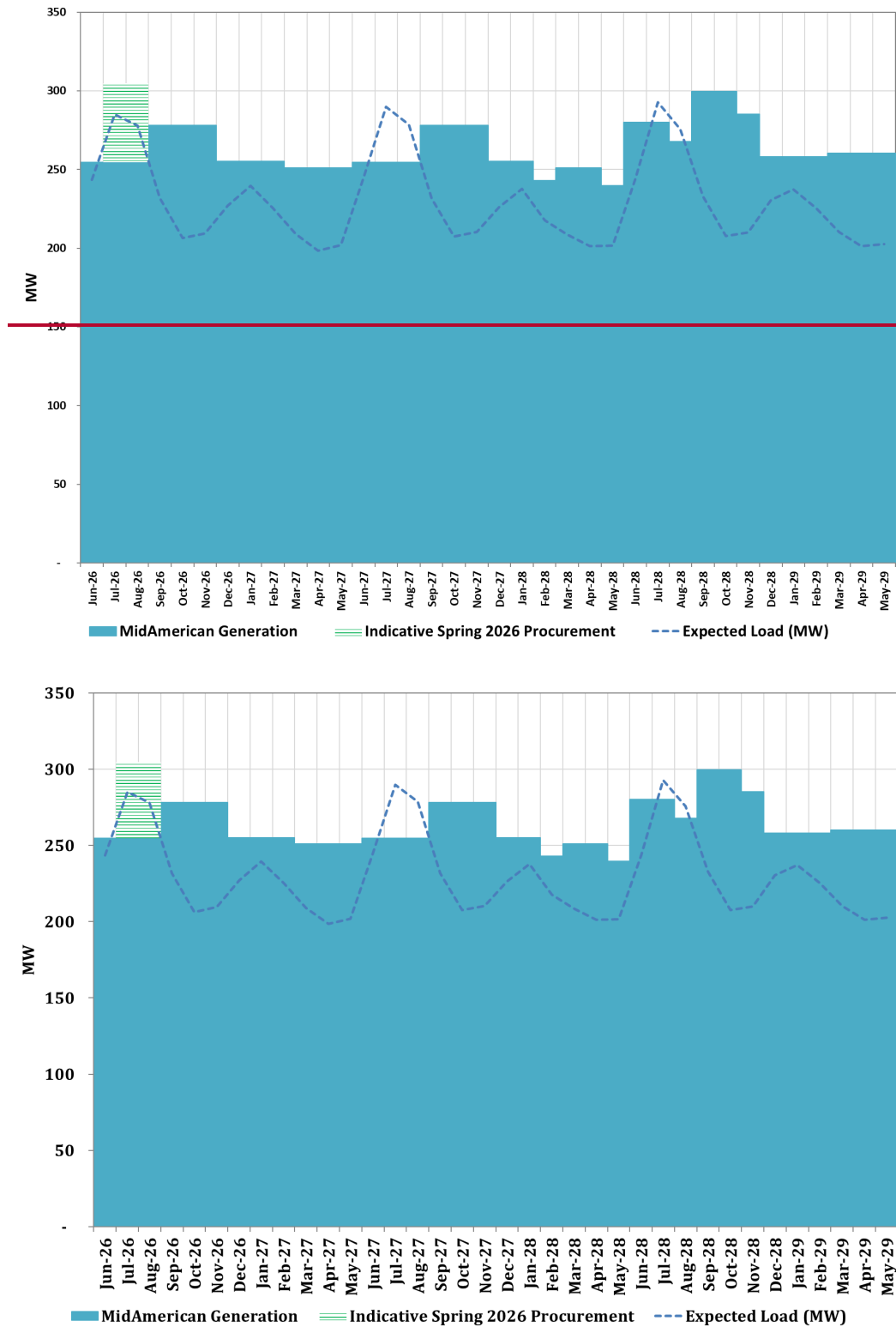
Figure 7-5: MidAmerican Peak Energy Supply Portfolio and Load 220
