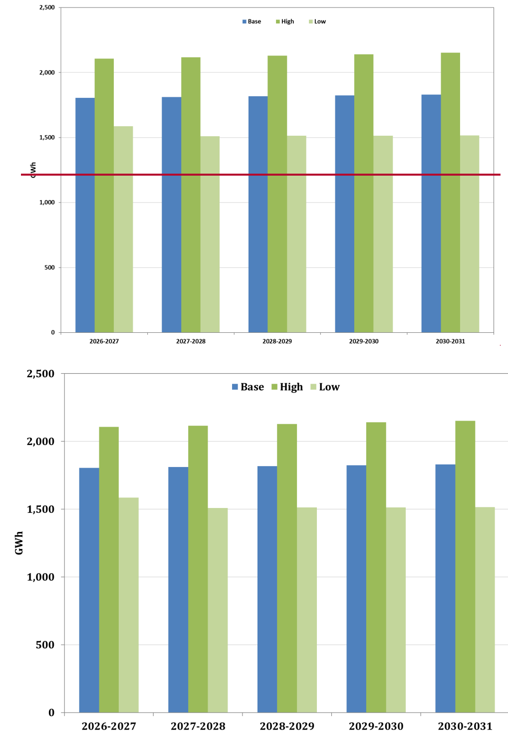
Figure 3-19: Supply Obligation in MidAmerican's Forecast Scenarios
