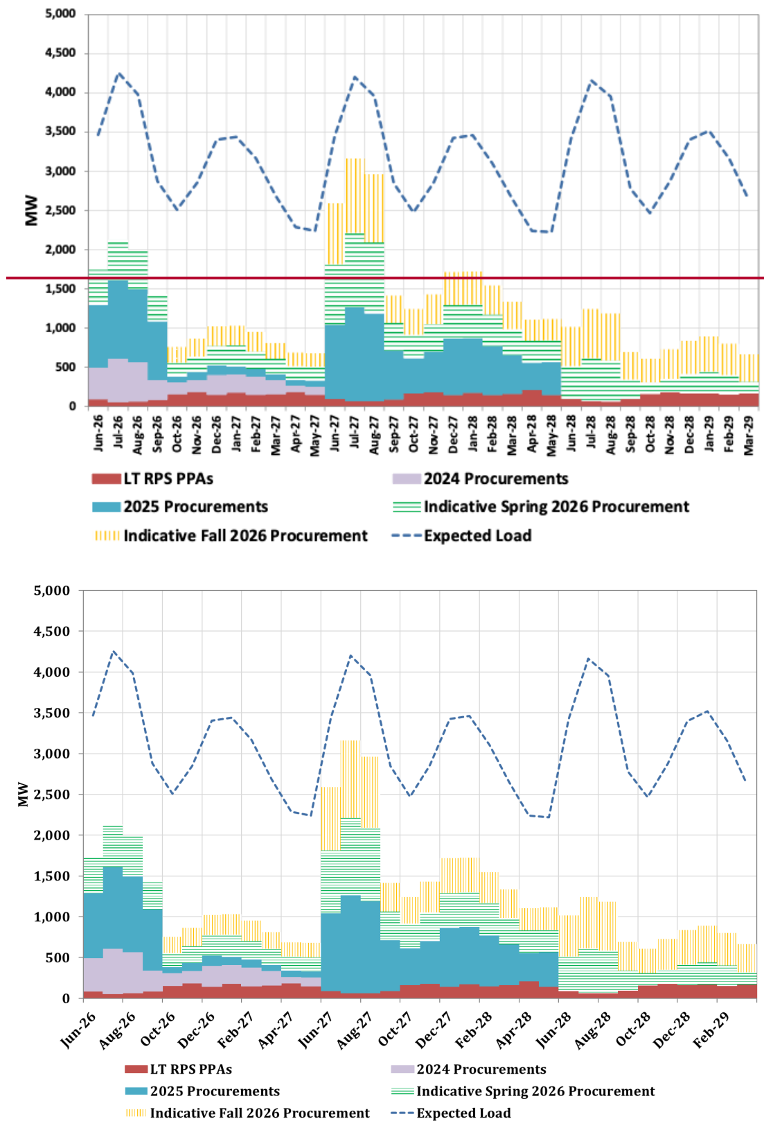
Figure 7-3: ComEd Peak Energy Supply Portfolio and Load
