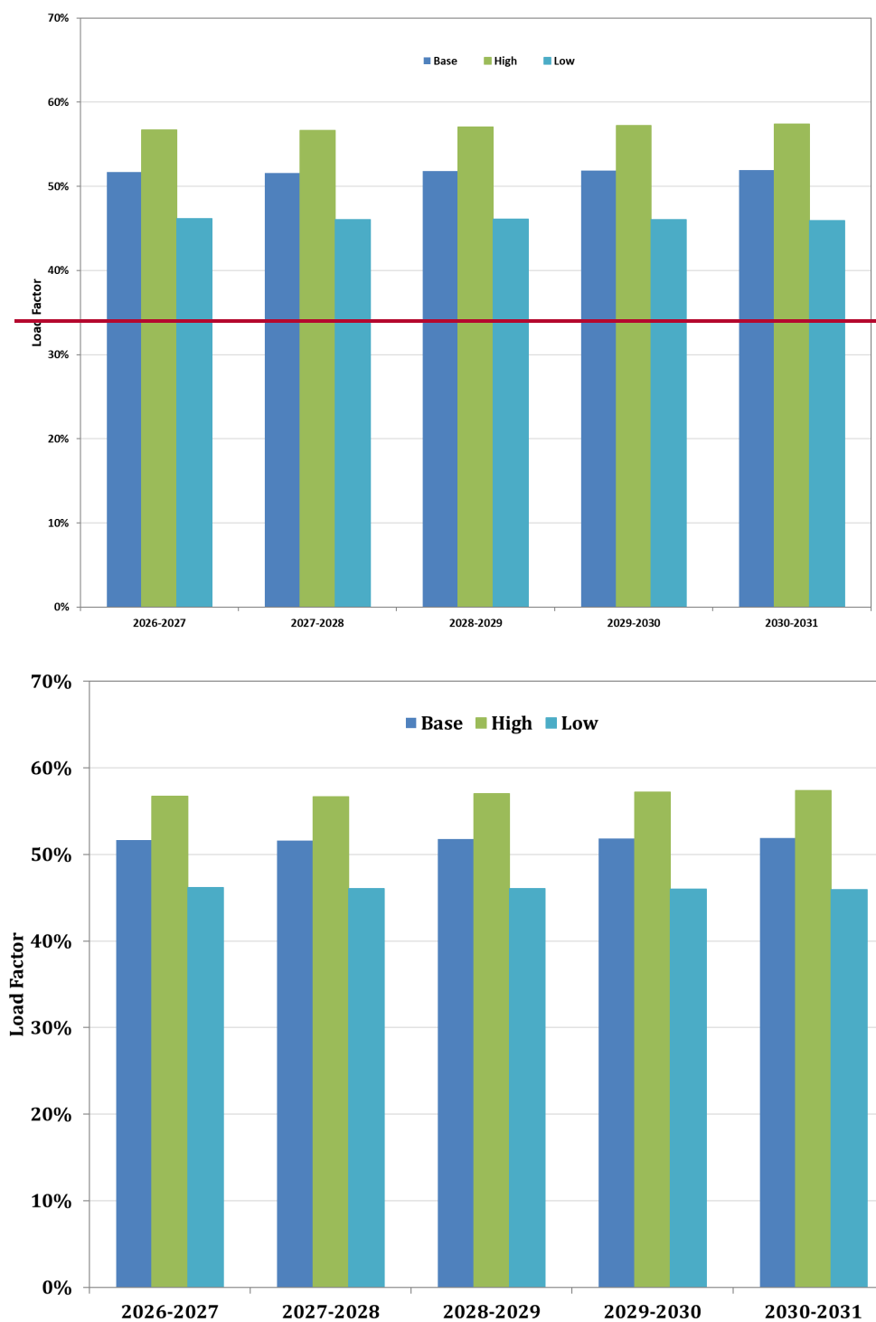
Figure 3-22: Load Factor in MidAmerican's Forecast Scenarios
