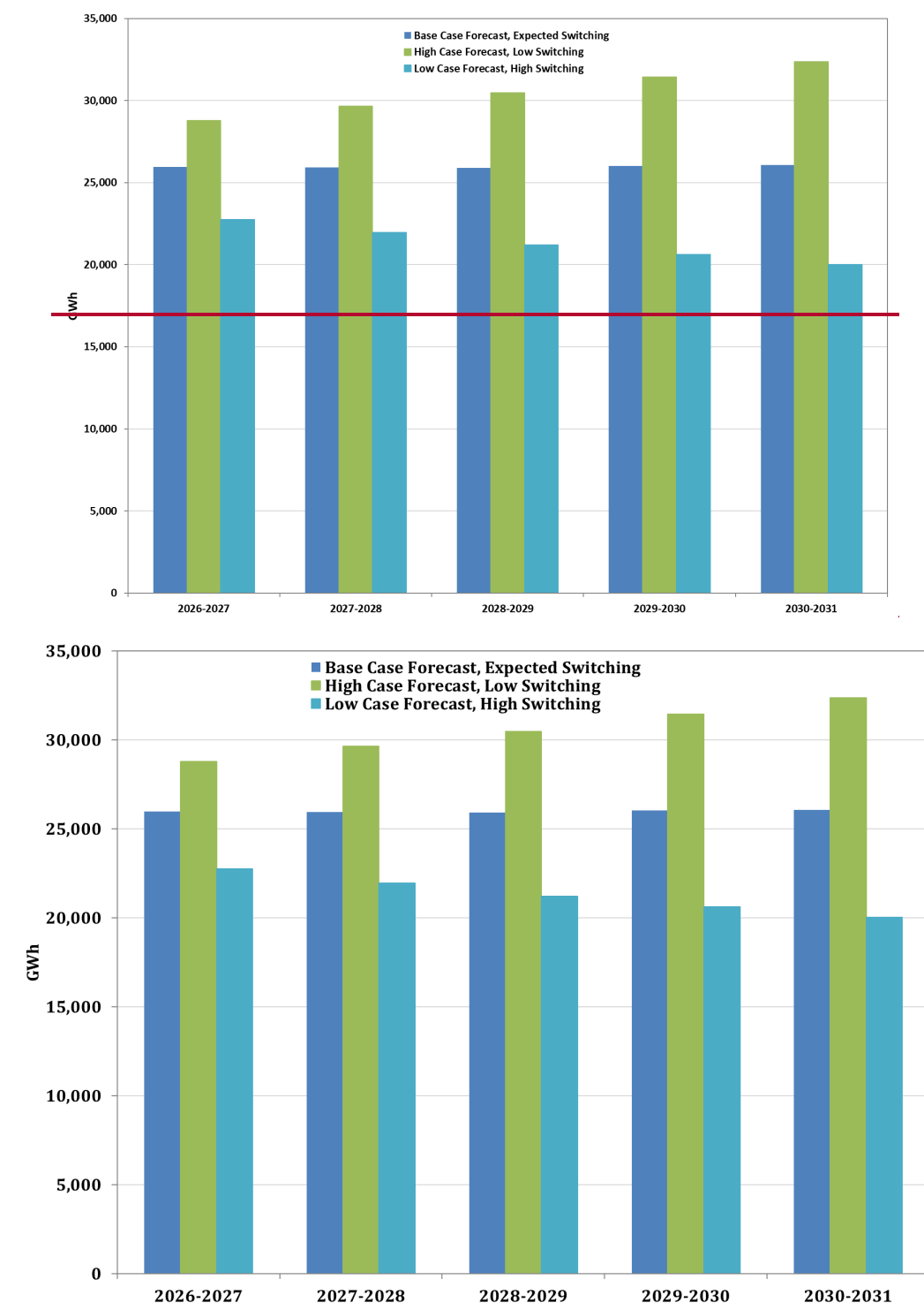
Figure 3-12: Supply Obligation in ComEd's Forecast Scenarios
