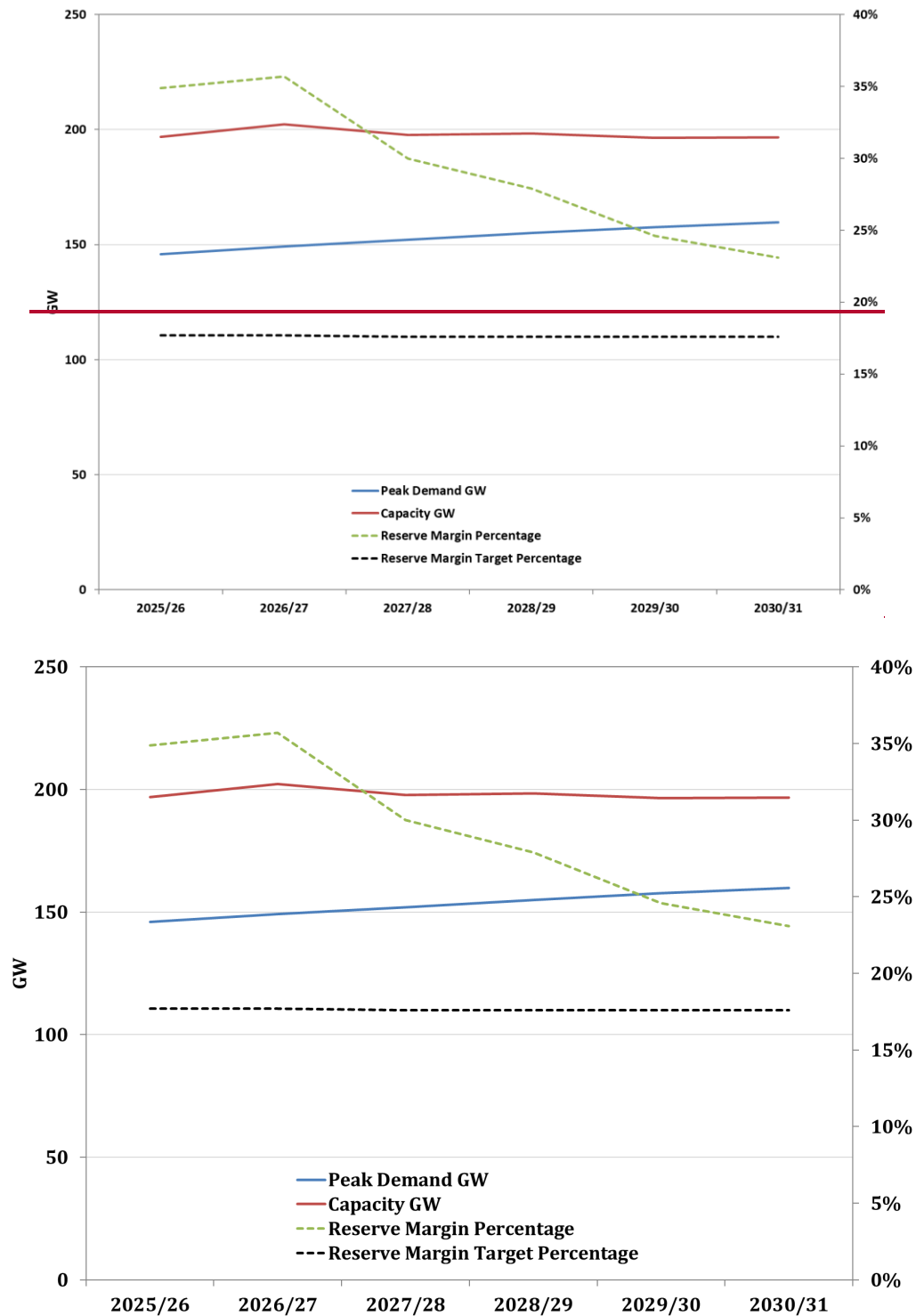
Figure 5-1: NERC Projection of Supply and Demand for Delivery Years 2025-2026 to 2030-2031
