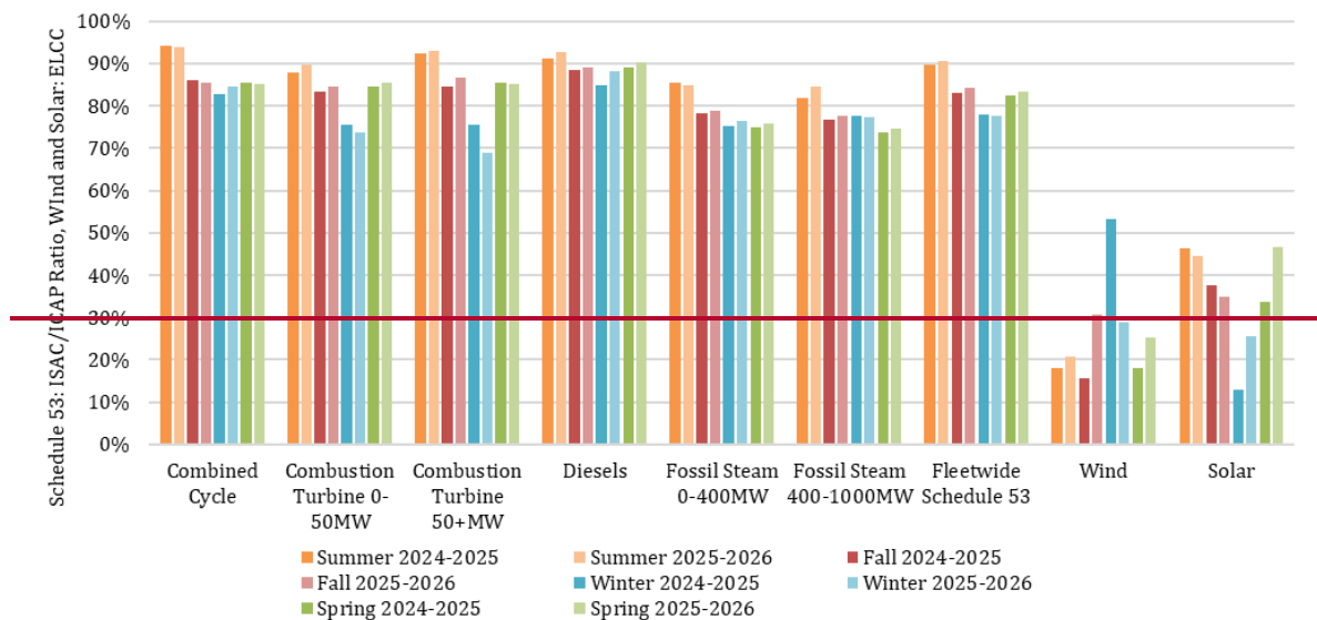
Figure 5-6: Schedule 53 Seasonal Resource ISAC/ICAP; Wind and Solar ELCCs ELCCs 166
