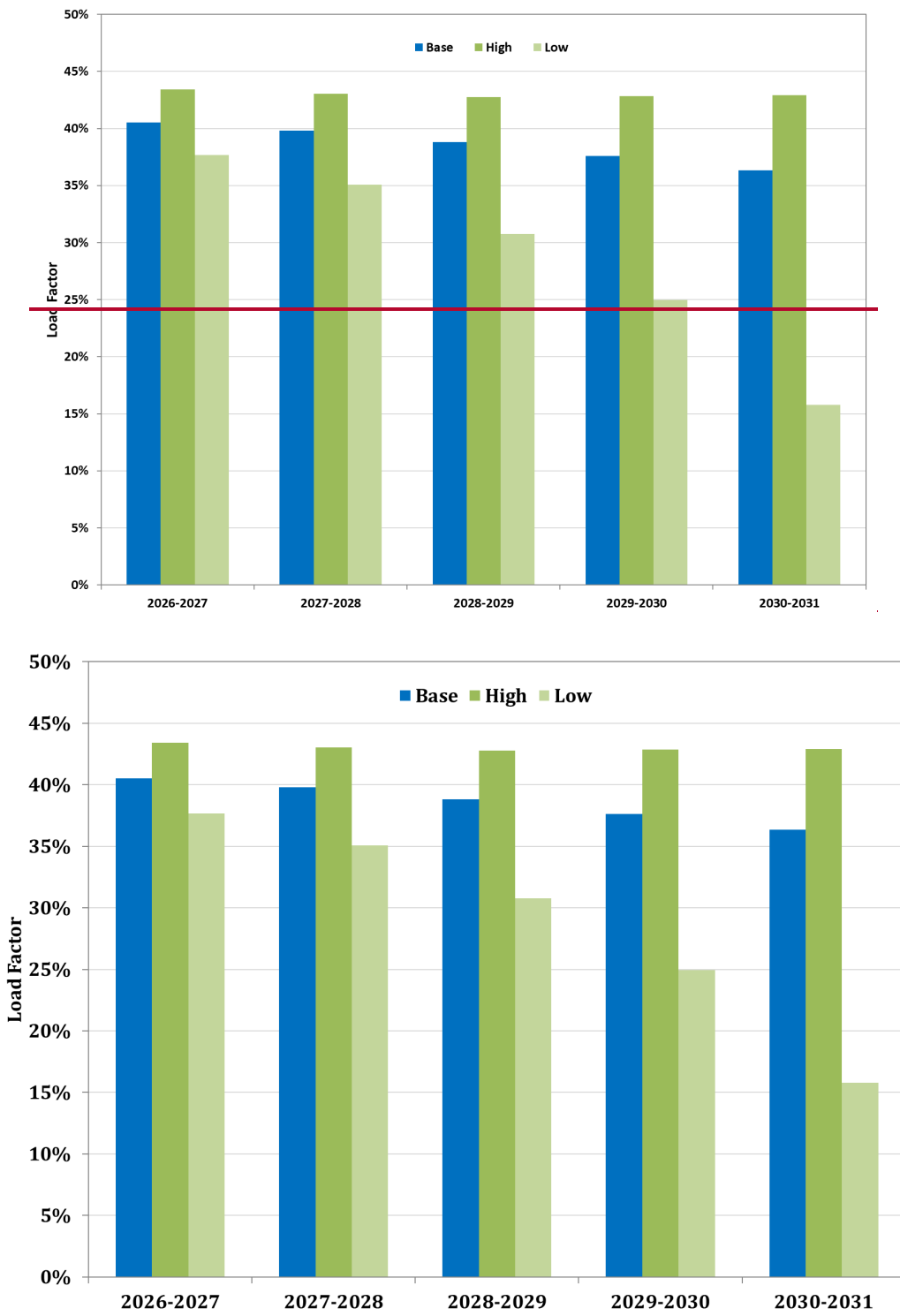
Figure 3-7: Load Factor in Ameren Illinois' Forecast Scenarios
