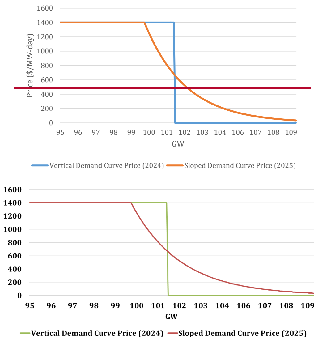
Figure 5-10: Comparison of Vertical vs Sloped Demand Curves for MISO PRA (Zone 4 2024 / North Central 2025)
