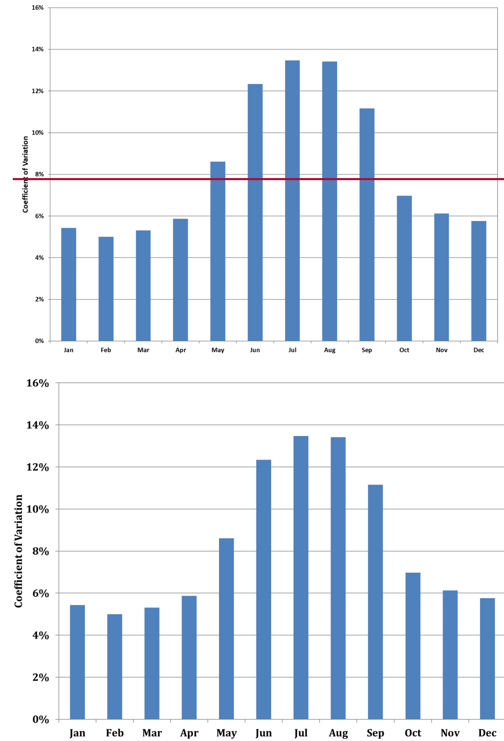
Figure 3-23: Coefficient of Variation of Daily Peak-Period Loads
