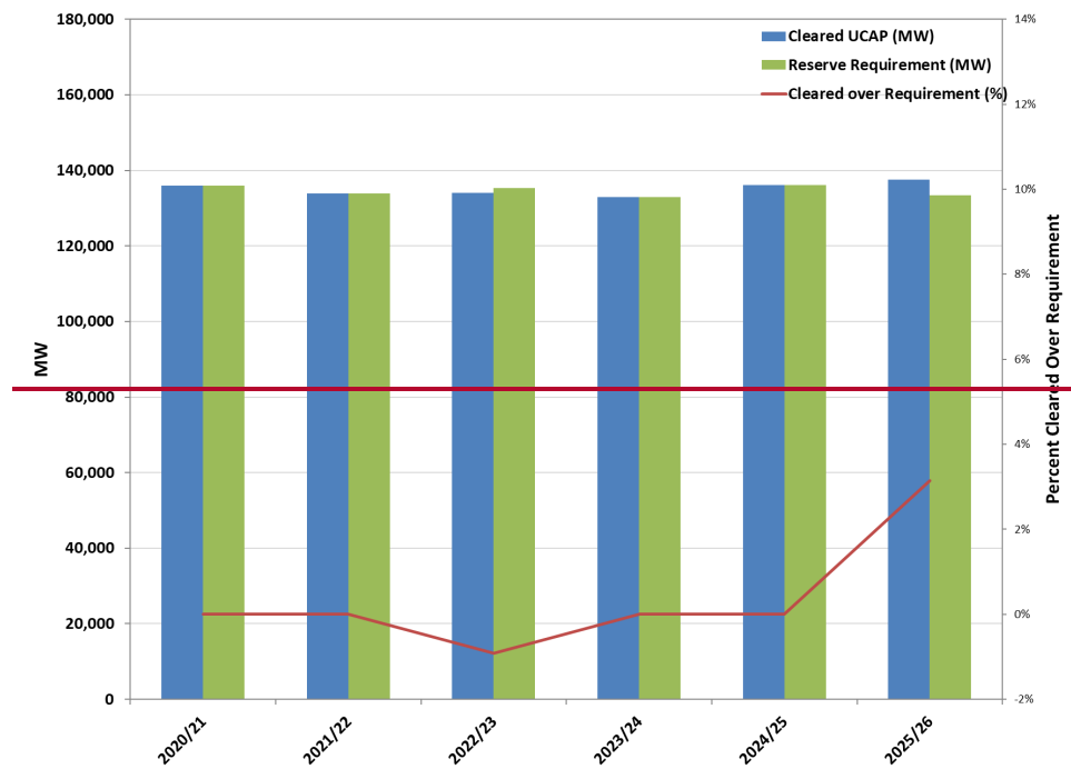
Figure 5-4: MISO Historical PRA Cleared UCAP and Reserve Margin
