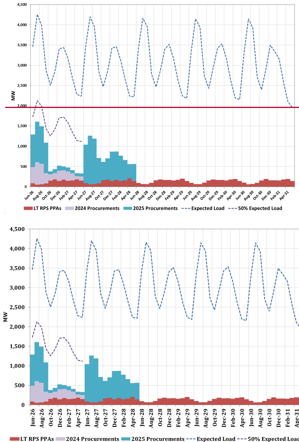
Figure 4-2: ComEd's On-Peak Supply Gap - June 2026-May 2031 period - Base Case Load Forecast
