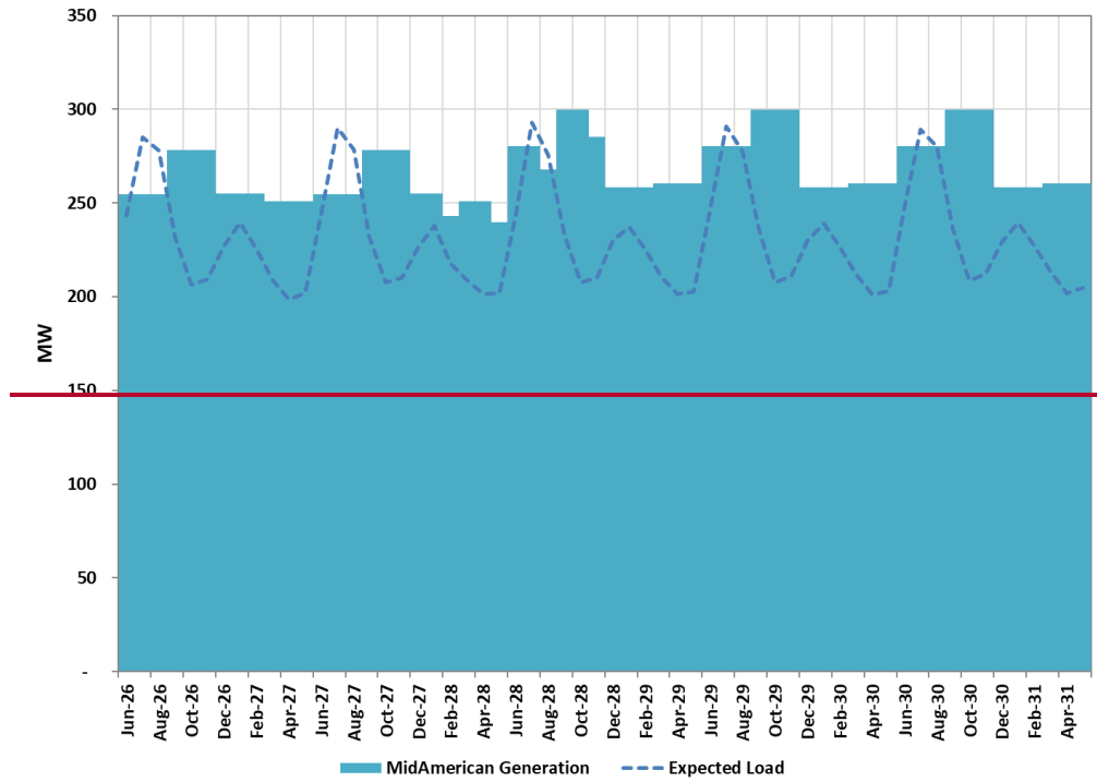
Figure 4-3: MidAmerican's On-Peak Supply Gap - June 2026-May 2031 period - Base Case Load Forecast
