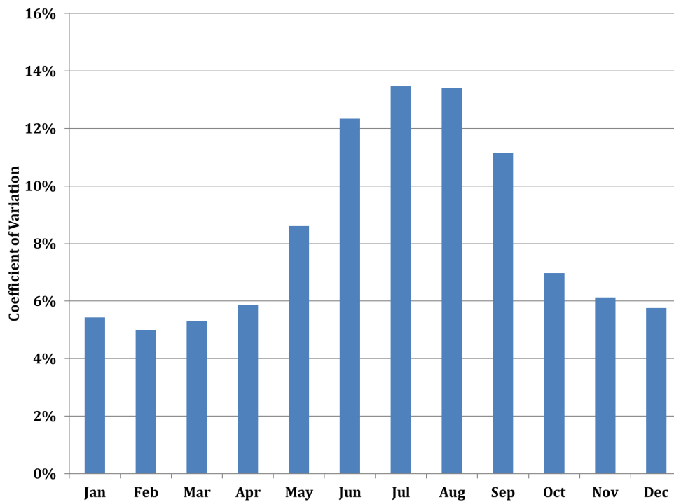
Figure 3-23: Coefficient of Variation of Daily Peak-Period Loads
