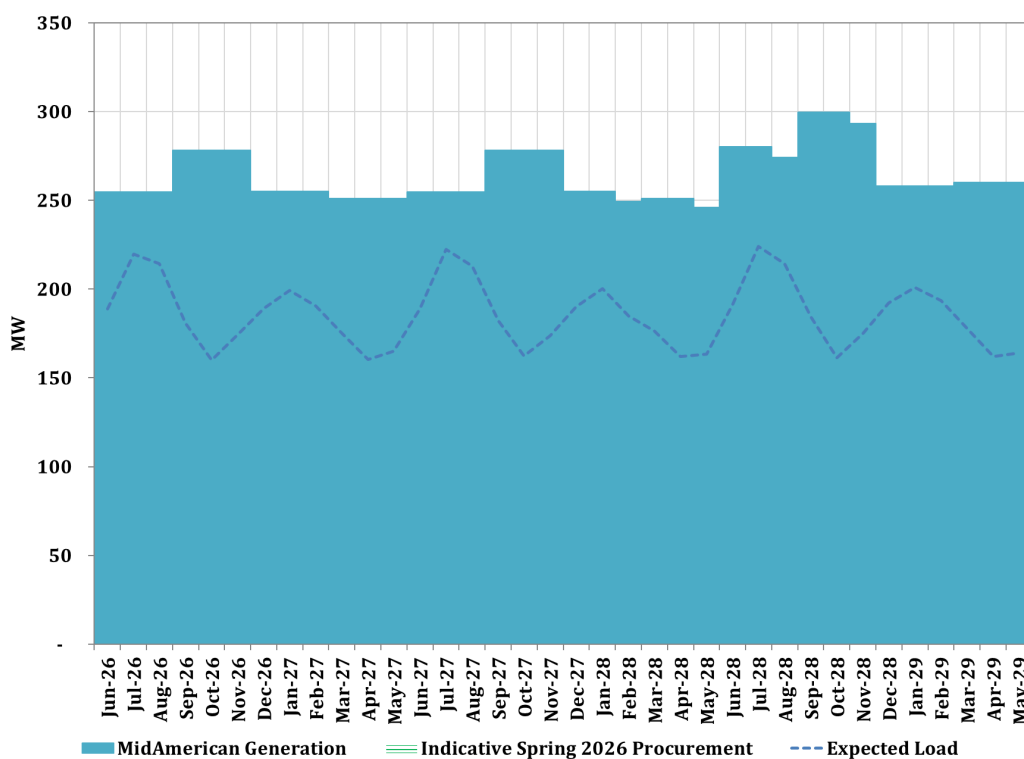
Figure 7-6: MidAmerican Off-Peak Energy Supply Portfolio and Load
