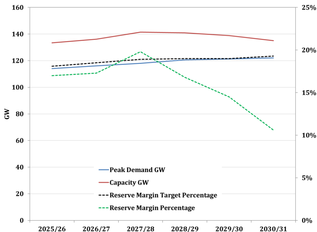
Figure 5-3: NERC Projection of Supply and Demand for the Delivery Years 2025-2026 to 2030-2031 135
