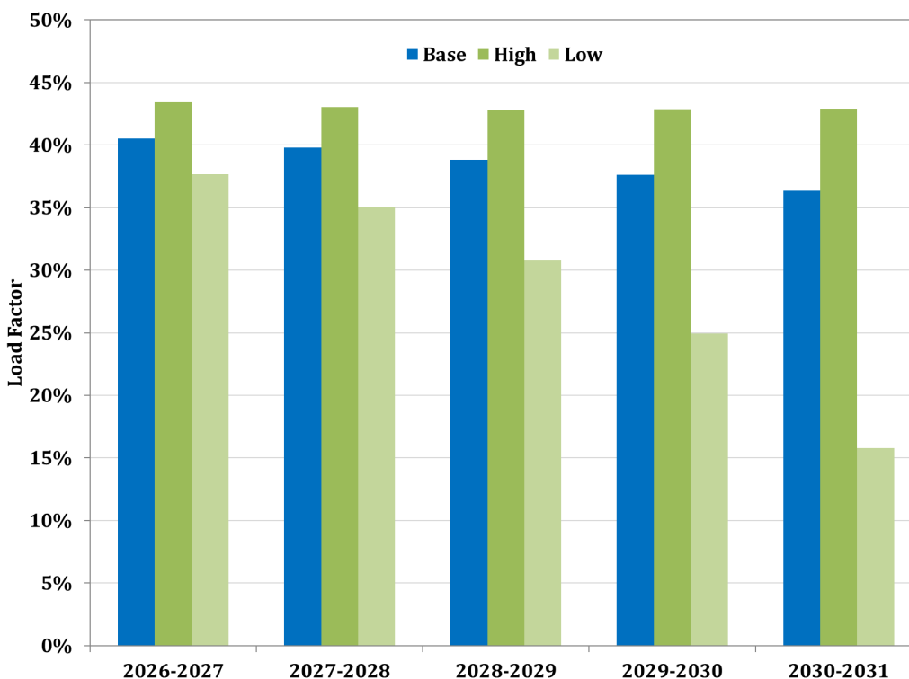
Figure 3-7: Load Factor in Ameren Illinois' Forecast Scenarios
