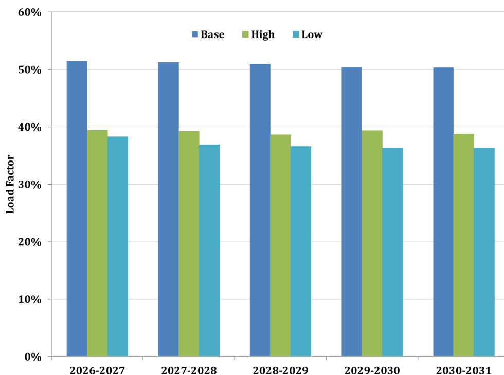
Figure 3-15: Load Factor in ComEd's Forecasts Scenarios
