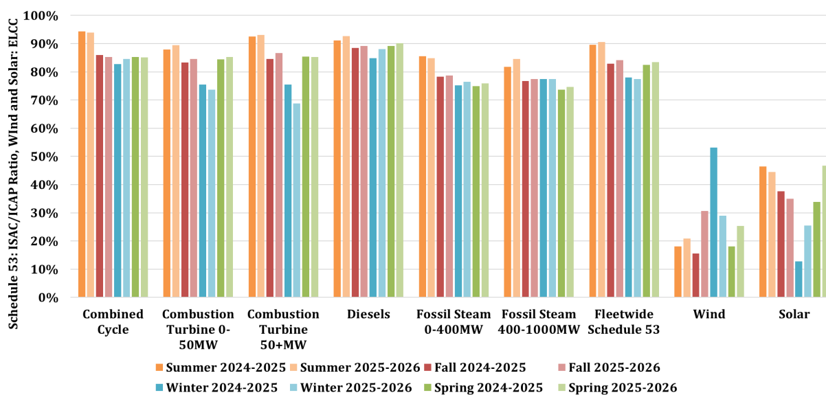
Figure 5-6: Schedule 53 Seasonal Resource ISAC/ICAP; Wind and Solar ELCCs 161
