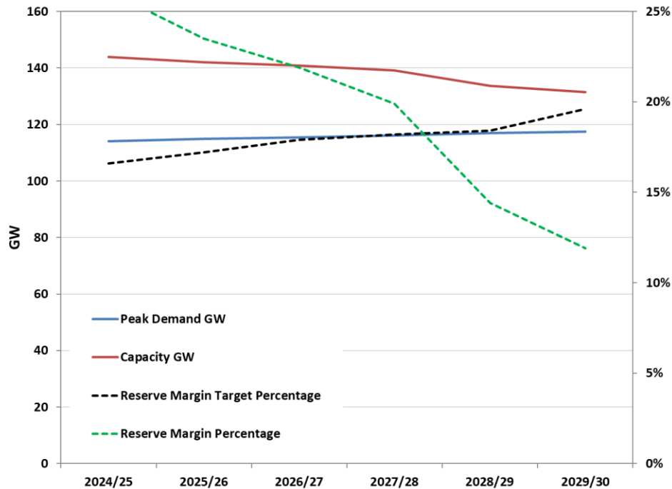
Figure 5-2: NERC Projection of Supply and Demand in MISO for the Delivery Years 2024-2025 to 2029-2030
