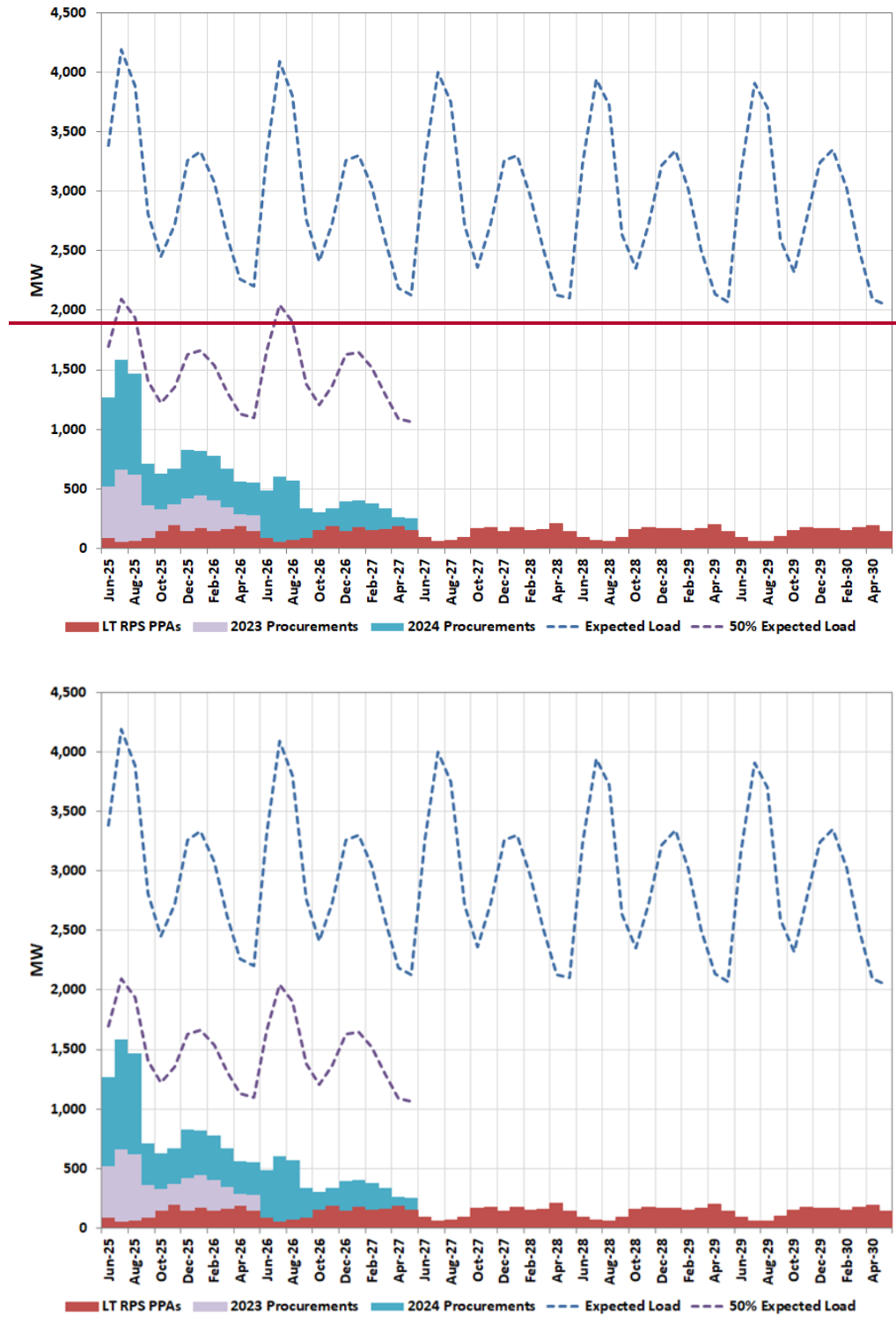
Figure 4-2: ComEd's On-Peak Supply Gap - June 2025-May 2030 period - Base Case Load Forecast
