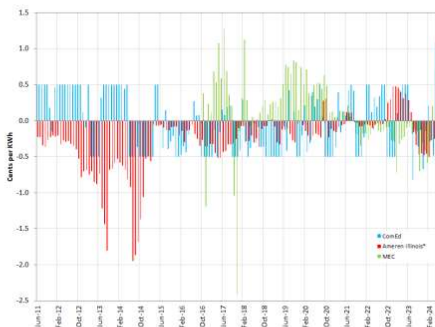
Figure 6-1: Purchased Electricity Adjustments in Cents/kWh, June 2011 – June 2024
