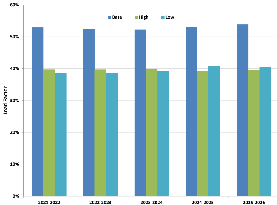
Figure 3-15: Load Factor in ComEd's Forecasts
