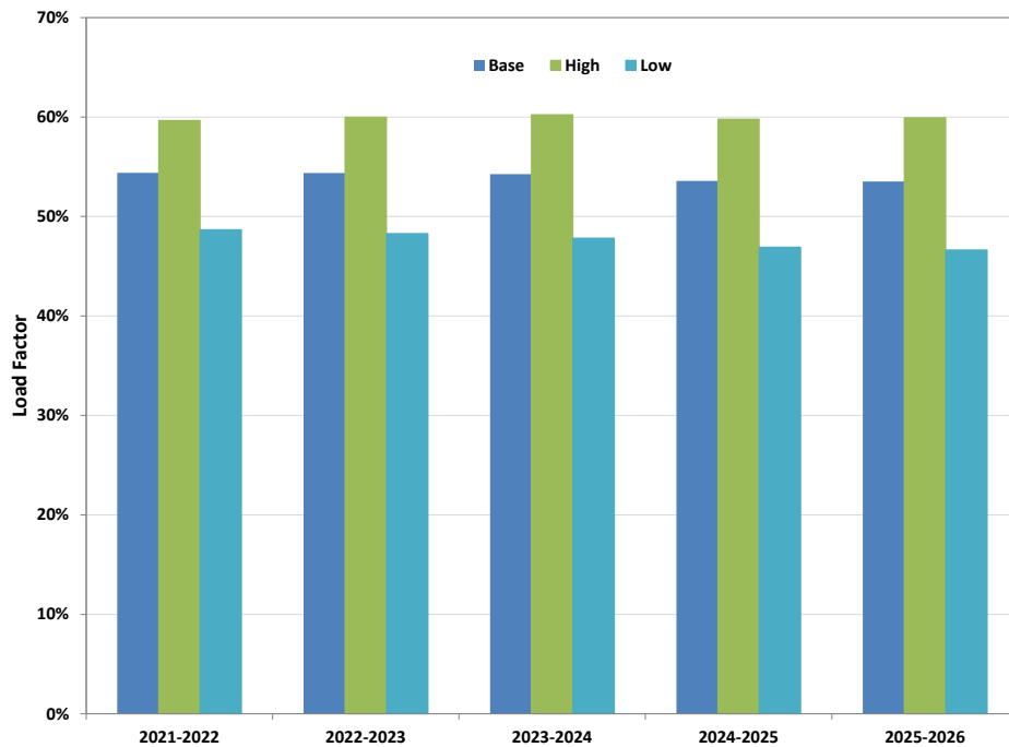
Figure 3-22: Load Factor in MidAmerican's Forecasts
