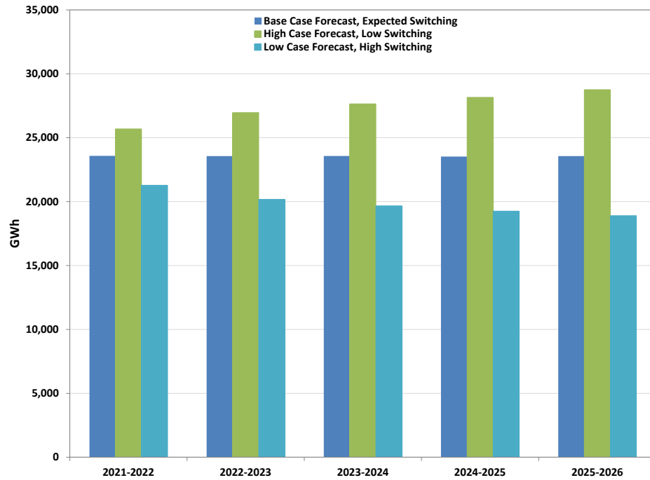
Figure 3-12: Supply Obligation in ComEd's Forecasts
