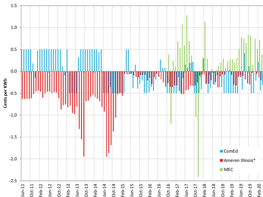
Figure 6-1: Purchased Electricity Adjustments in Cents/kWh, June 2011 – May 2020
