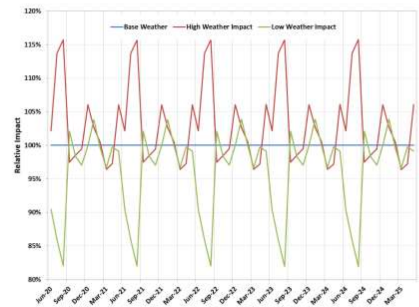
Figure 3-11: The Impact of Weather in ComEd's Forecasts
