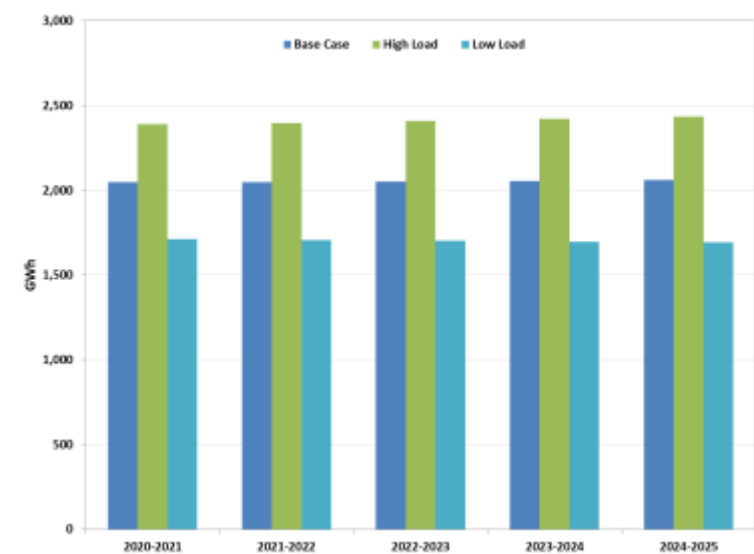
Figure 3-19: Supply Obligation in MidAmerican's Forecasts
