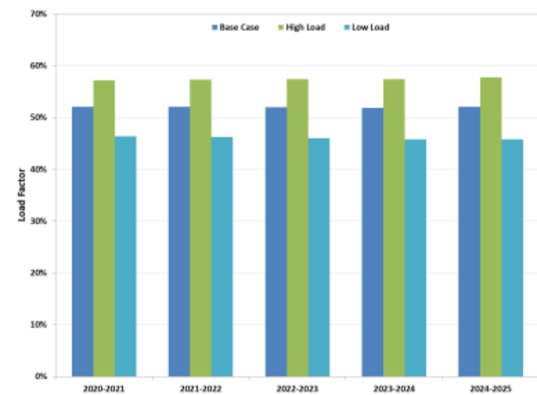
Figure 3-22: Load Factor in MidAmerican's Forecasts
