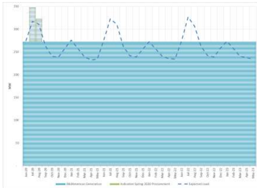
Figure 7-5: MidAmerican Peak Energy Supply Portfolio and Load 172
