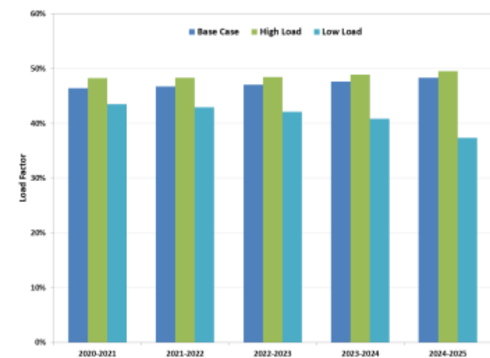
Figure 3-7: Load Factor in Ameren Illinois' Forecasts
