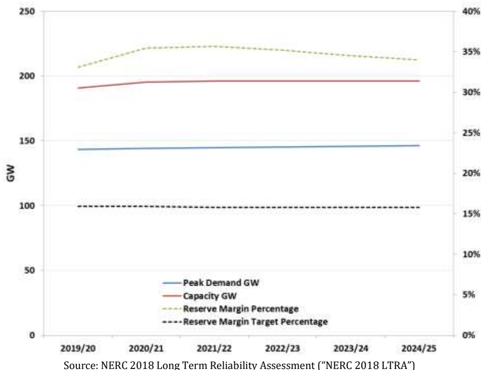
Figure 5-1: PJM / NERC Projected Capacity Supply and Demand for Delivery Years 2019-2020 to 2024-2025
