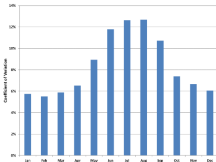
Figure 3-23: Coefficient of Variation of Daily Peak-Period Loads
