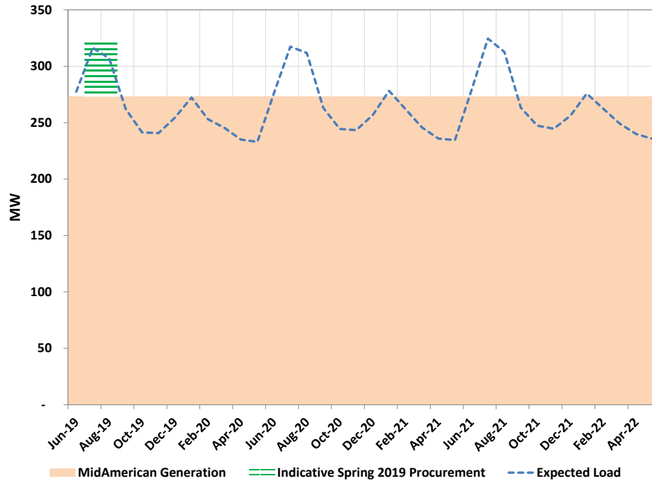
Figure 7-5: MidAmerican Peak Energy Supply Portfolio and Load 151
