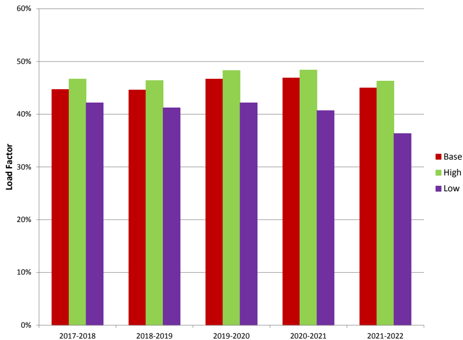
Figure 3-9: Load Factor in Ameren Illinois' Forecasts
