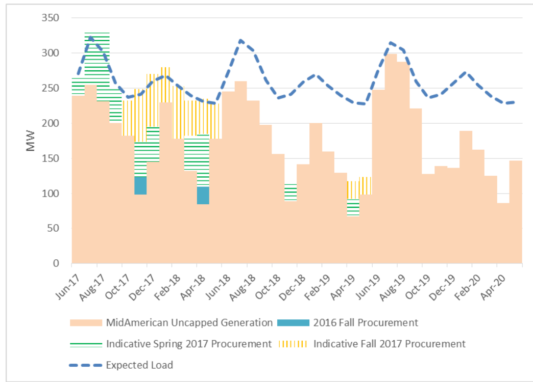
Figure 7-5 MidAmerican Peak Uncapped Energy Supply Portfolio and Load
