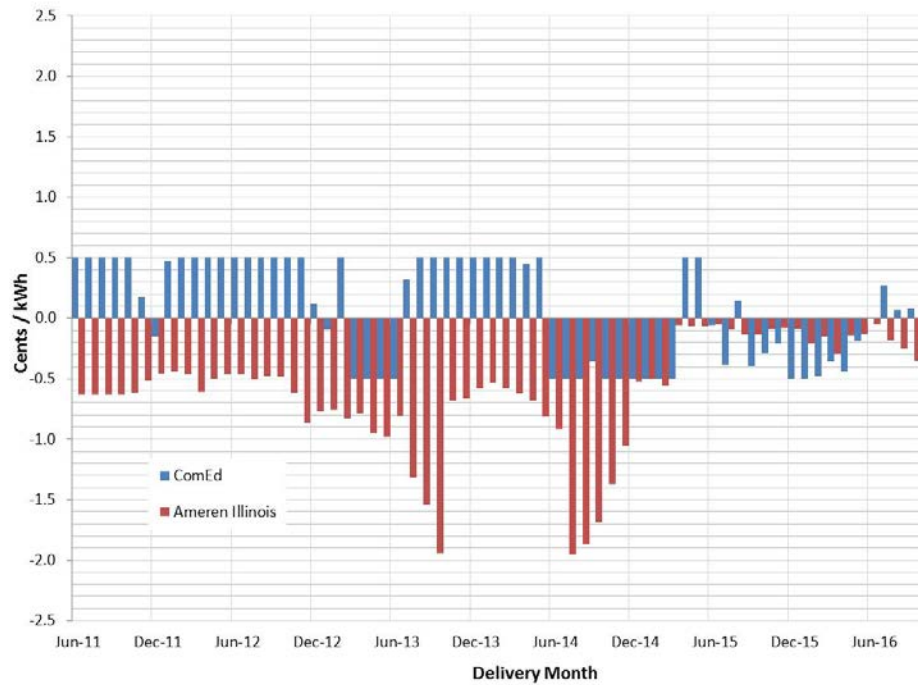
Figure 6-1: Purchased Electricity Adjustments in Cents/kWh, June 2011 – September August 2016
