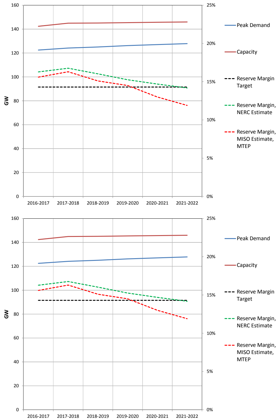
Figure 5-3: MISO NERC Projected Capacity Supply and Demand for the Planning Years 2016-2017 to 2021-2022
