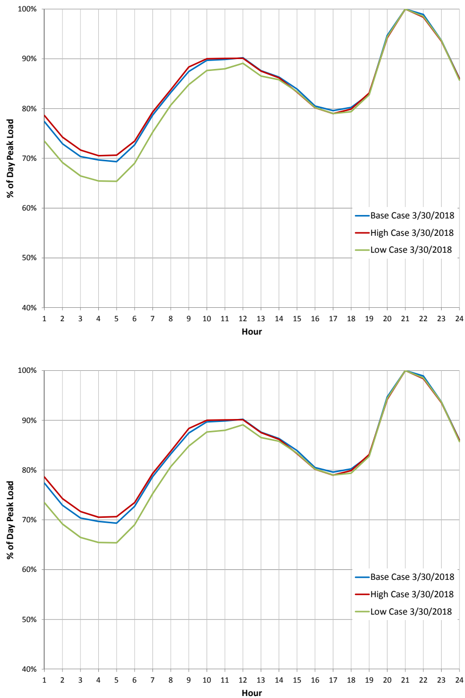
Figure 3-16: Sample Daily Load Shape, Spring Day in ComEd's Forecasts
