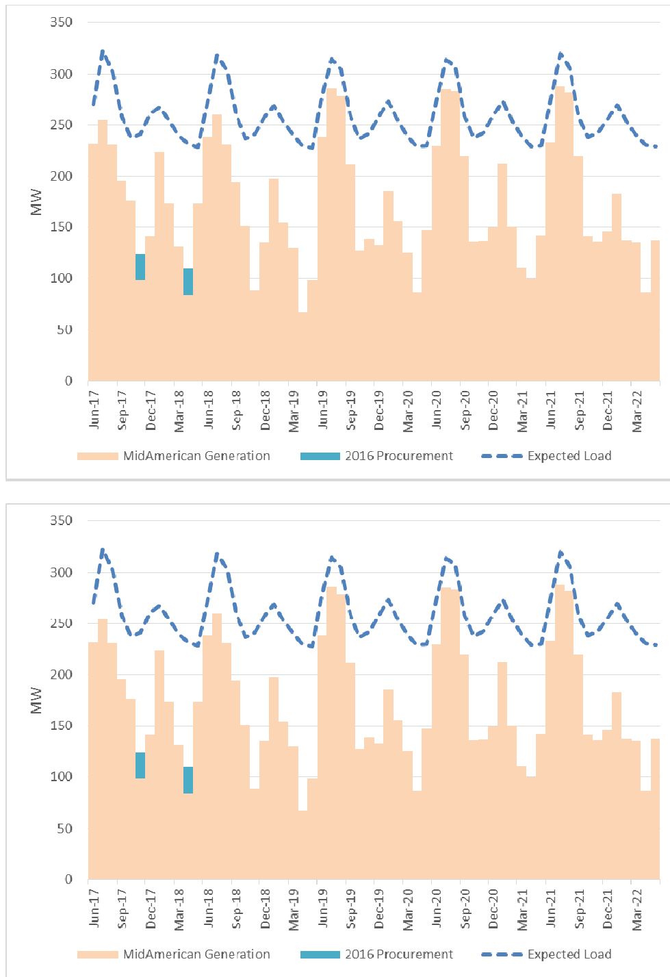
Figure 4-3: MidAmerican's On-Peak Supply Gap - June 2017-May 2022 period - Base Case Load Forecast
