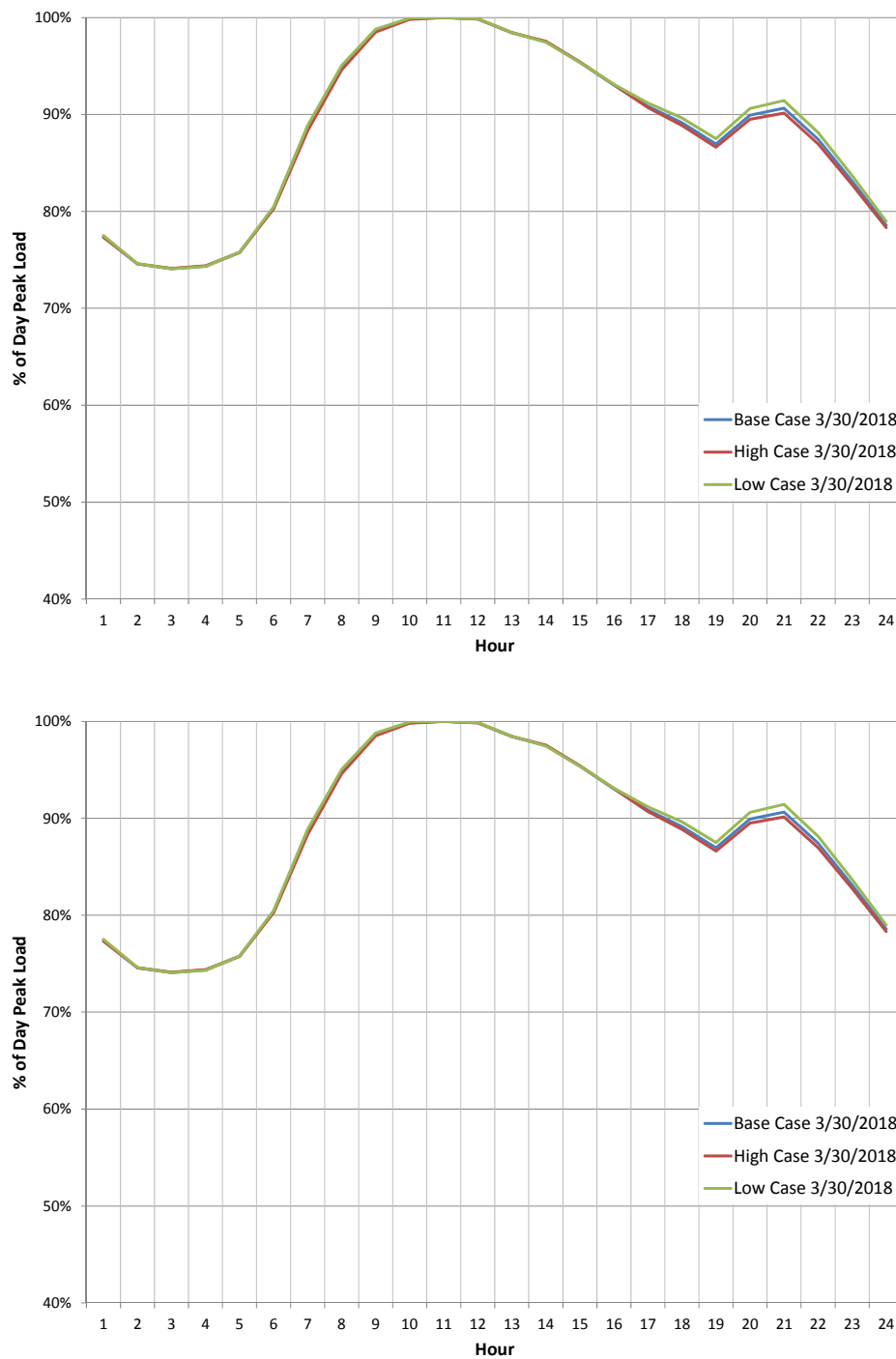
Figure 3-23: Sample Daily Load Shape, Spring Day in MidAmerican's Forecasts
