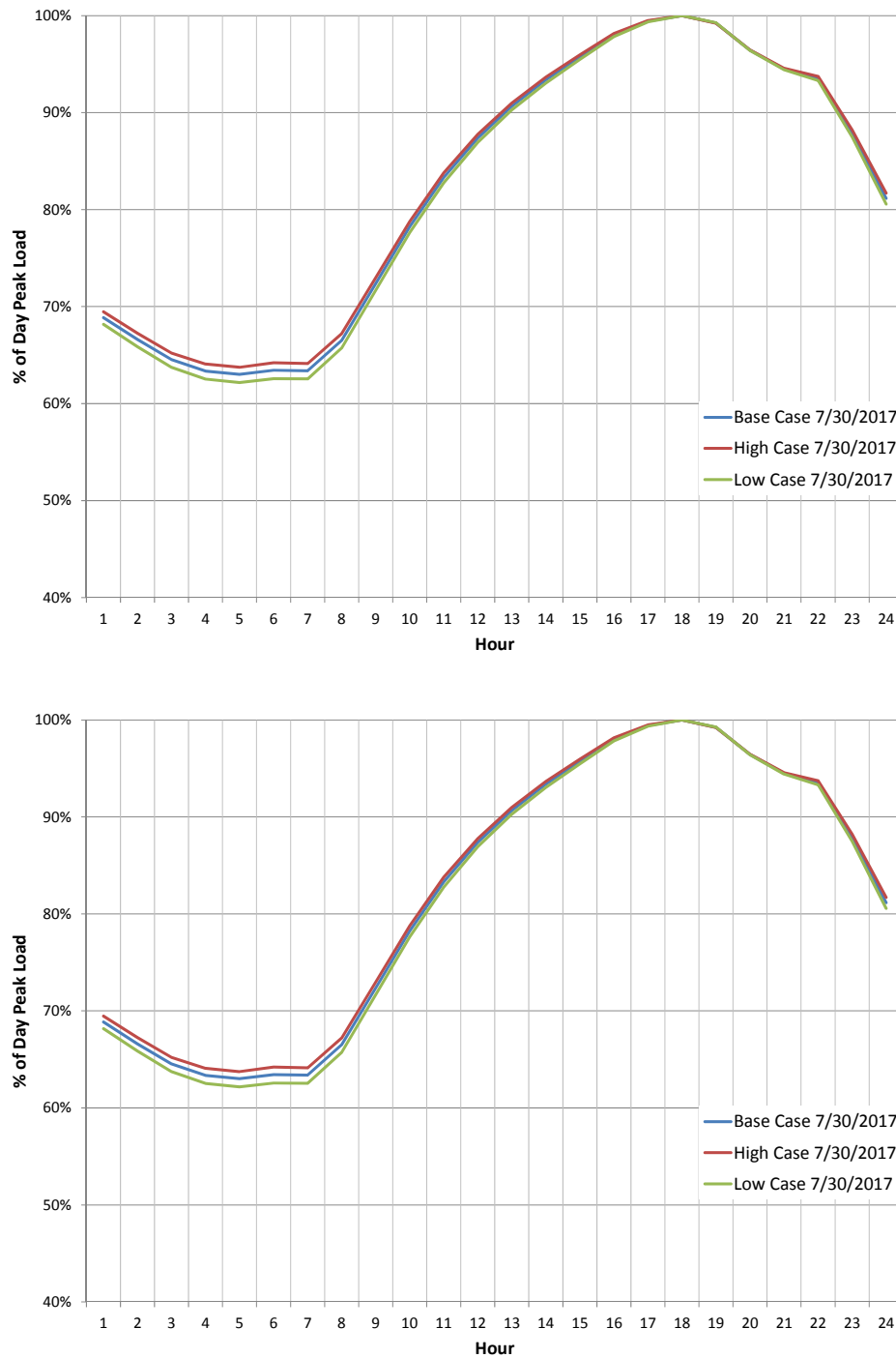
Figure 3-22: Sample Daily Load Shape, Summer Day in MidAmerican's Forecasts
