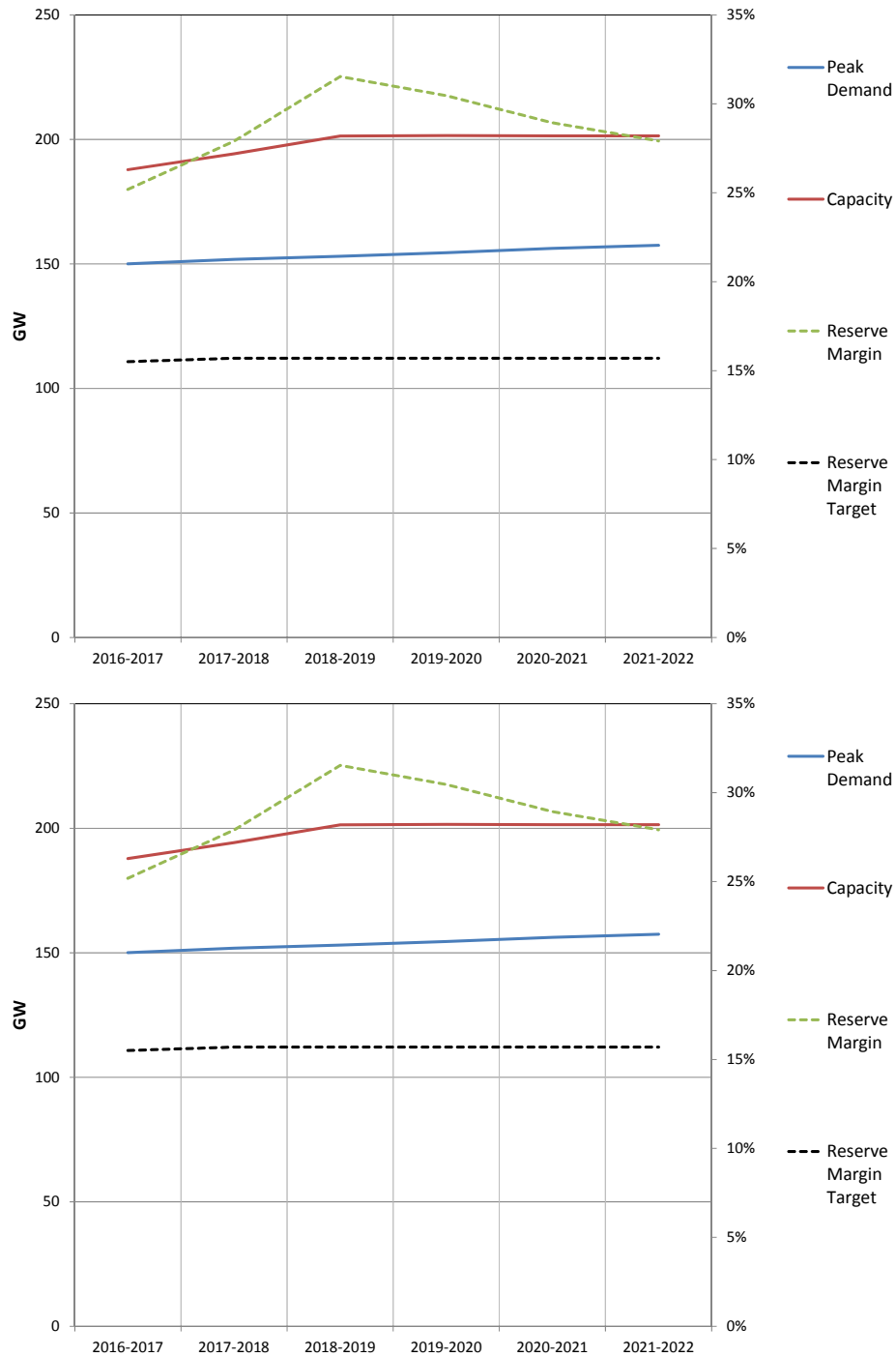
Figure 5-2: PJM NERC Projected Capacity Supply and Demand for Planning Years 2016-2017 to 2021-2022
