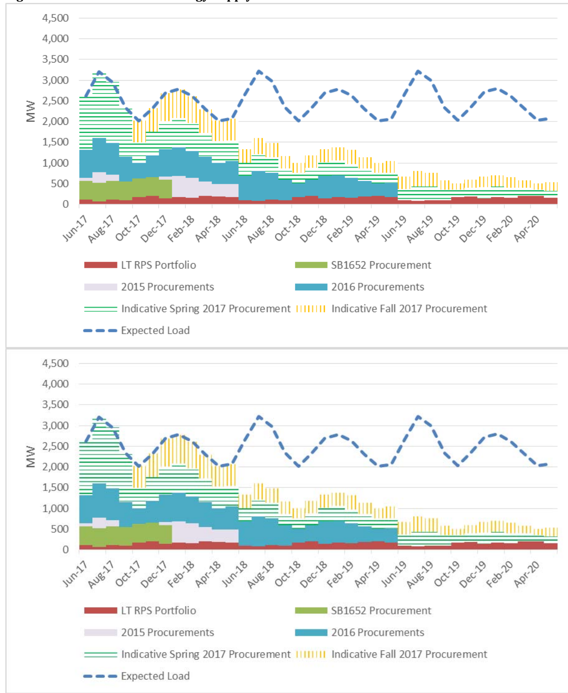
Figure 7-4 ComEd Off-Peak Energy Supply Portfolio and Load
