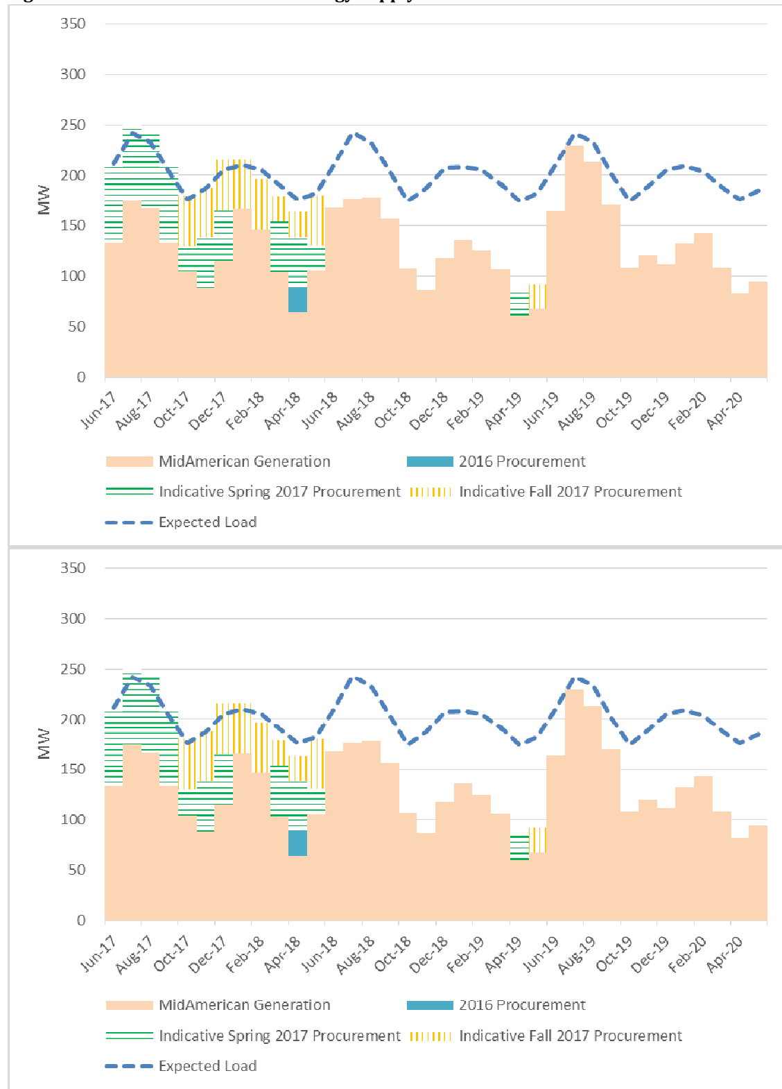
Figure 7-6 MidAmerican Off-Peak Energy Supply Portfolio and Load
