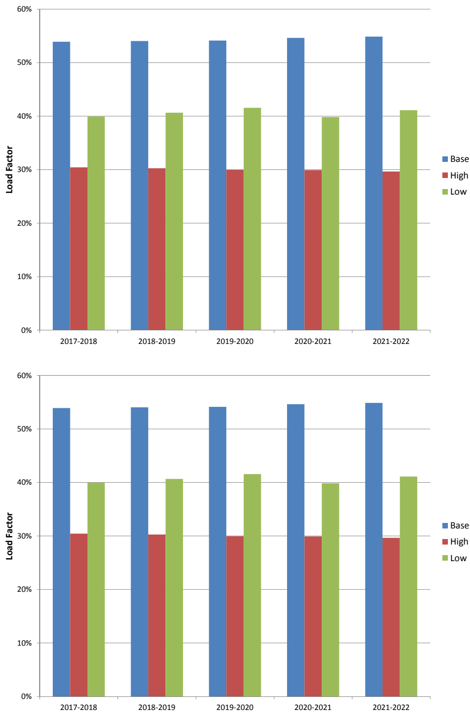
Figure 3-17: Load Factor in ComEd's Forecasts
