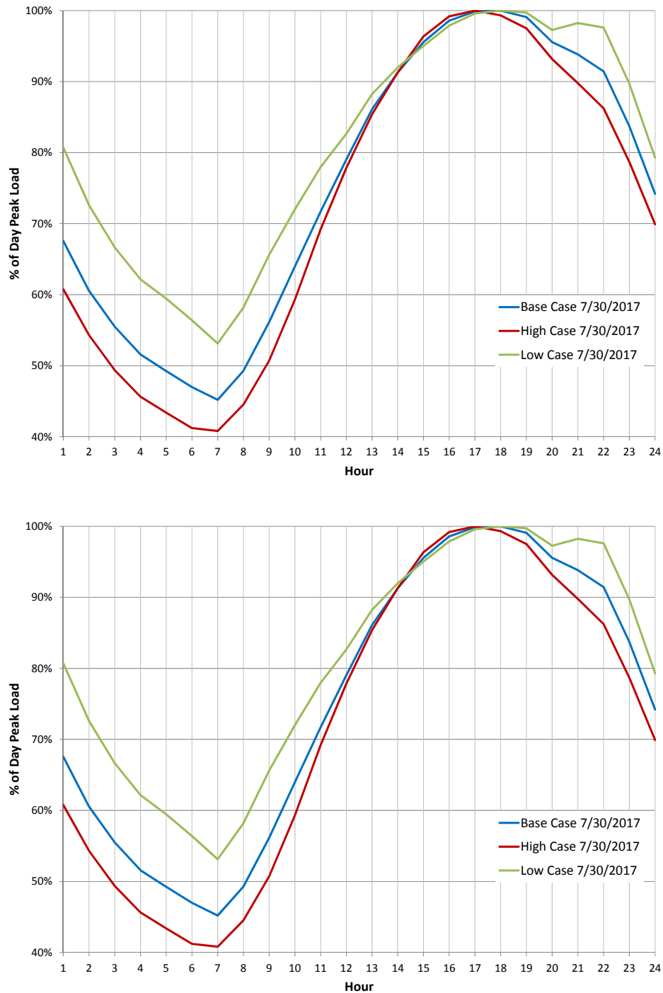
Figure 3-15: Sample Daily Load Shape, Summer Day in ComEd's Forecasts
