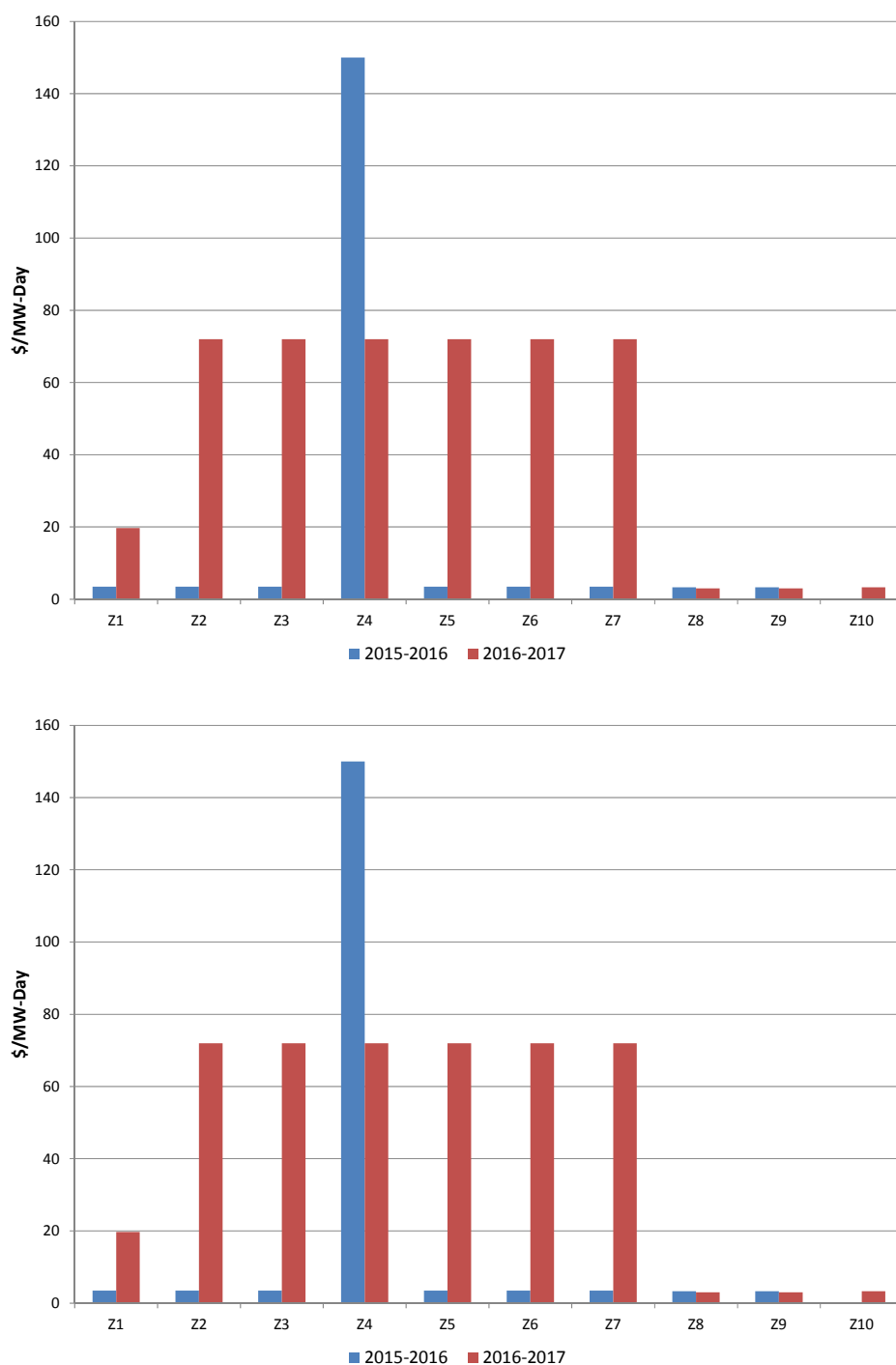
Figure 5-4: MISO PRA Results for Planning Years 2015-2016 and 2016-2017
