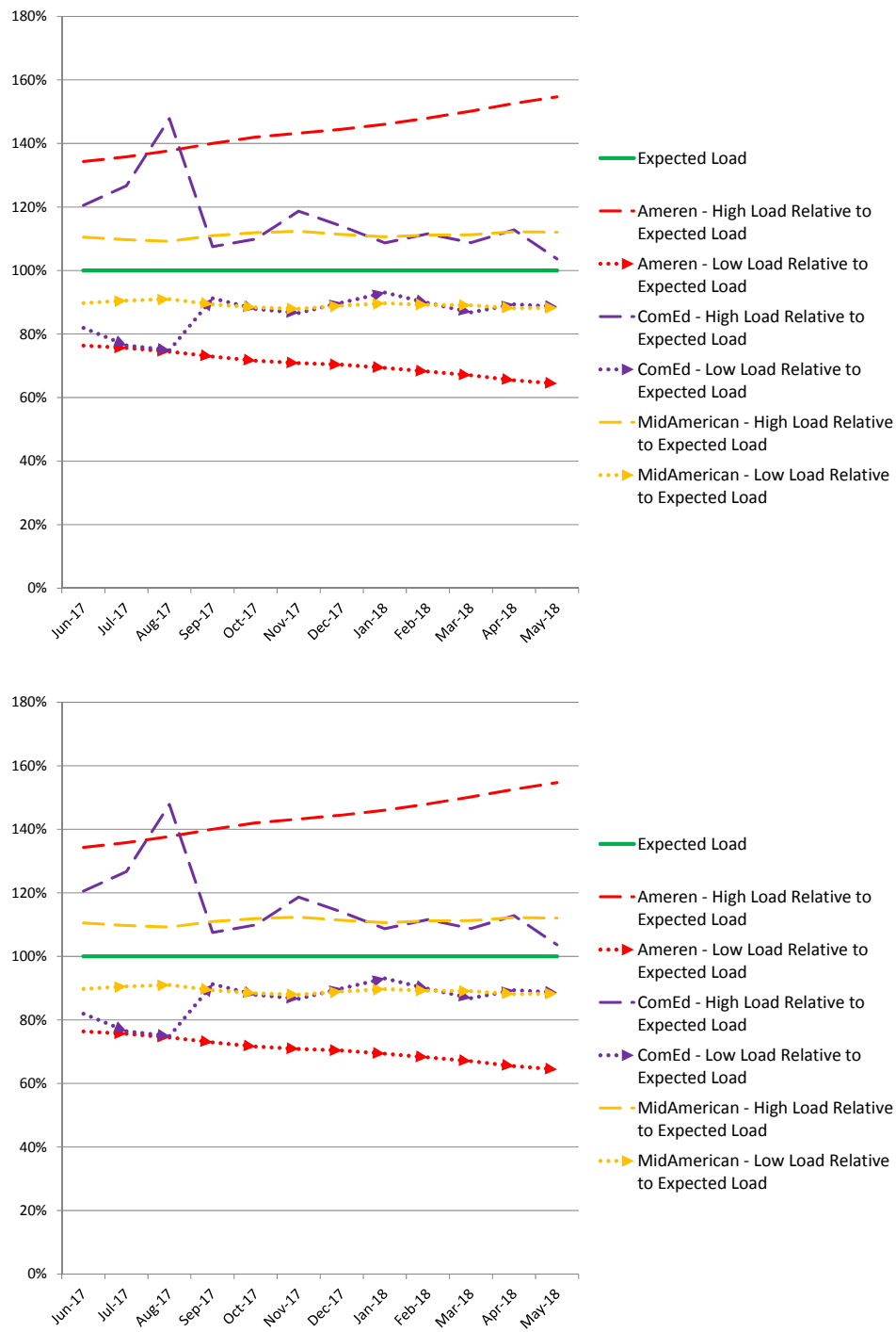
Figure 3-27: Comparison of Ameren Illinois, ComEd, and MidAmerican High and Low Forecasts for Delivery Year 2017-2018
