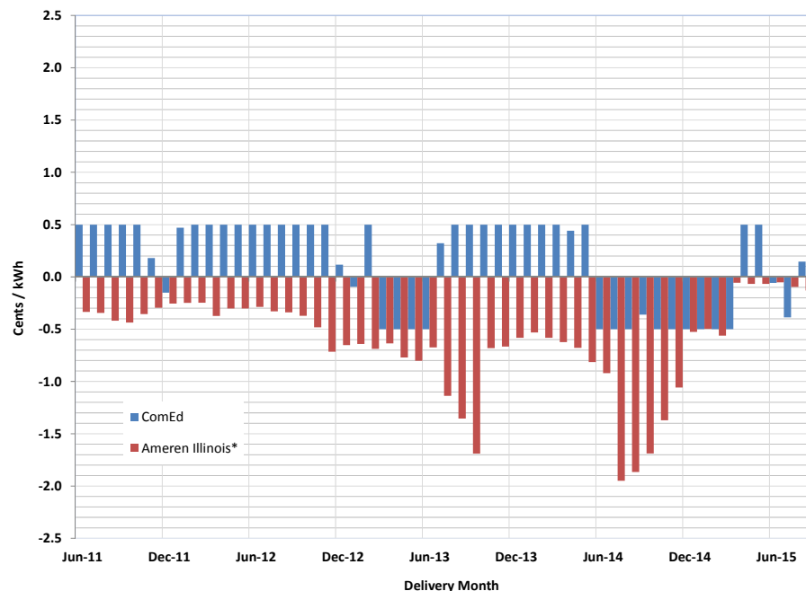
Figure 6-1: Purchased Electricity Adjustments in Cents/kWh, June 2011 – August October 2015
