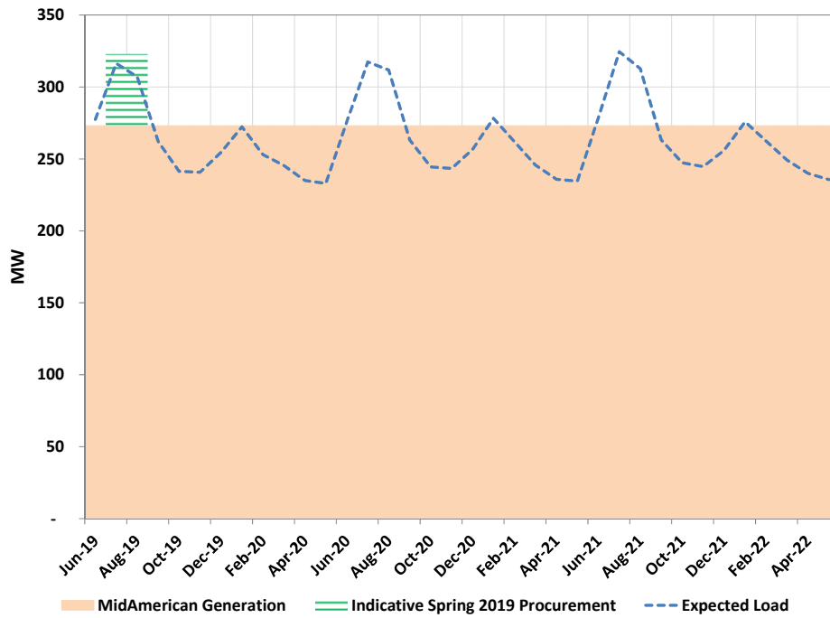
Figure 7-5: MidAmerican Peak Energy Supply Portfolio and Load 151
