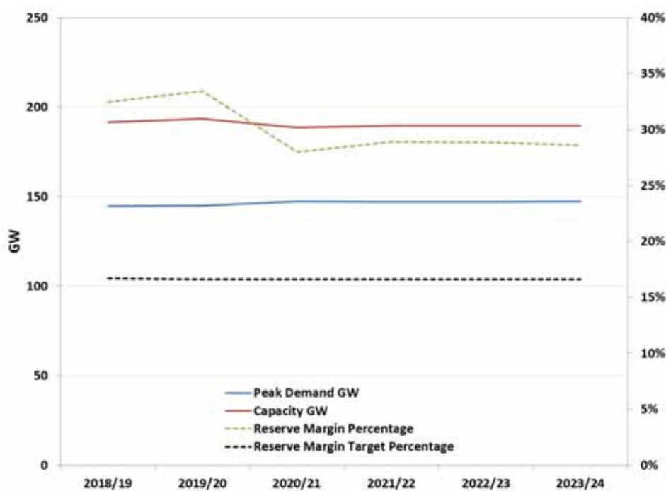
Figure 5-1: PJM NERC Projected Capacity Supply and Demand for Delivery Years 2018-2019 to 2023-2024
